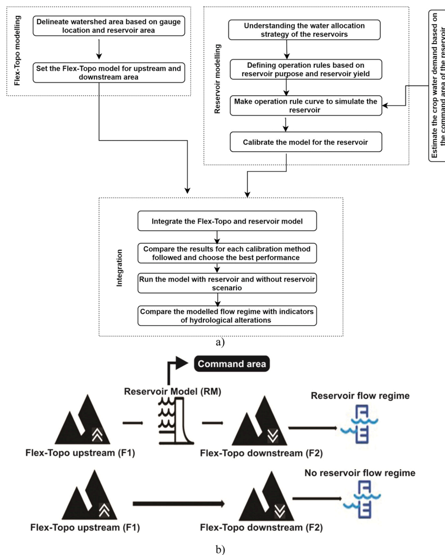
Fig. 3. (a) Overall methodology for analyzing the impact of reservoirs on flow regimes. (b) Modelling concept: Upstream and downstream contributing areas of the gauging station (GS) are modelled as F1 and F2 respectively. The top row shows how the reservoir model (RM) that contributes to irrigating a certain Command area is integrated with F1 and F2 and calibrated. In order to simulate the pre-dam situation, RM is removed from the calibrated model, along with its contribution to irrigate the Command area.
