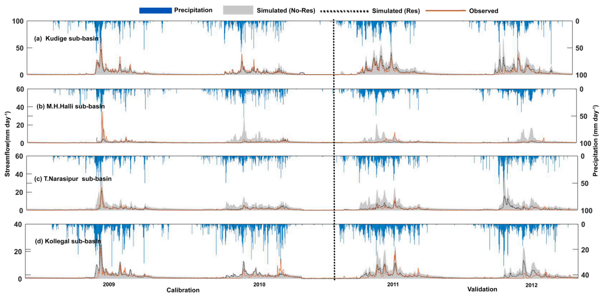
Fig. 9. The F-R-F model performance for the four sub-basins. Only four years (2009–2012) are presented here and the plots for the entire calibration and validation periods are given in S.5 in the supplementary materials . Additionally, 'No-Res' represent simulations without reservoirs and 'Res' represent simulations with reservoirs.
