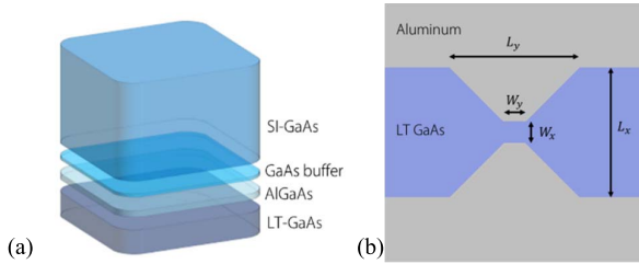
Fig. 6. (a) Dielectric stratification adopted for the device under investigation; the antenna is printed at the bottom side of the LT GaAs membrane. (b) Metal-lization bow-tie geometry printed over the photoconductor: W_x, W_y = 10 \mu\text{m} , L_x, L_y = 2 \text{ mm} , and taper angle of 90^\circ .
