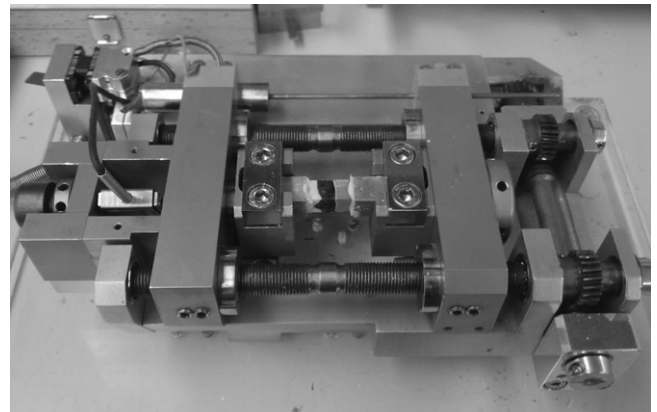
Figure 2. Meso-scale compression-tension test setup.
