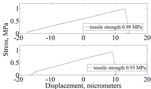
Figure 8. Meso-scale test results of cement paste-basalt aggregate interface.
