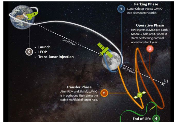
Fig. 1. LUMIO mission concept and phases.
