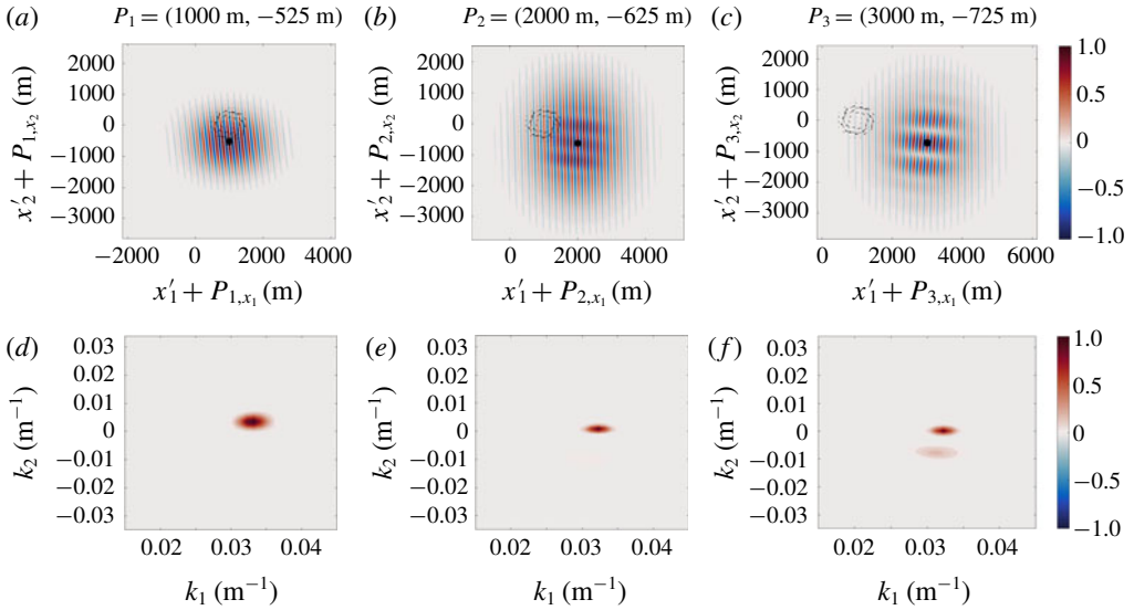
FIGURE 7. The evolution of the correlation function ( a–c ) and the corresponding action density spectrum ( d–f ) as presented by the spatial points P_1 , P_2 and P_3 . The values of the results are normalized by |\Gamma(P_j, \mathbf{x}')|_{\max} and |N(P_j, \mathbf{k})|_{\max} . These results were obtained for the simulation Ring 1 using SWAN.
