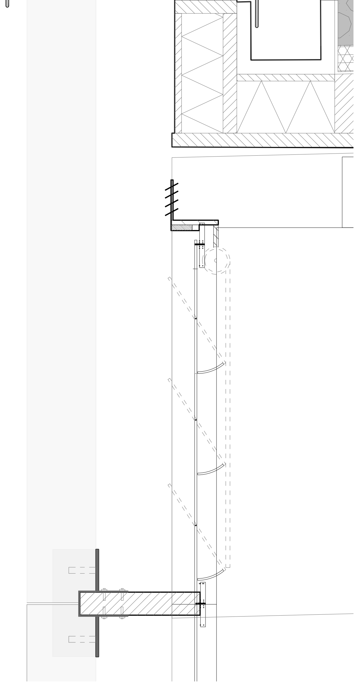
1:5 Detail B: gutter & glass vent detail
