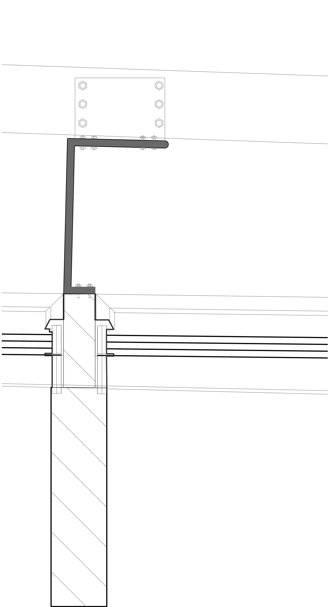
1:5 Detail A: Roof connection to glass ceiling
