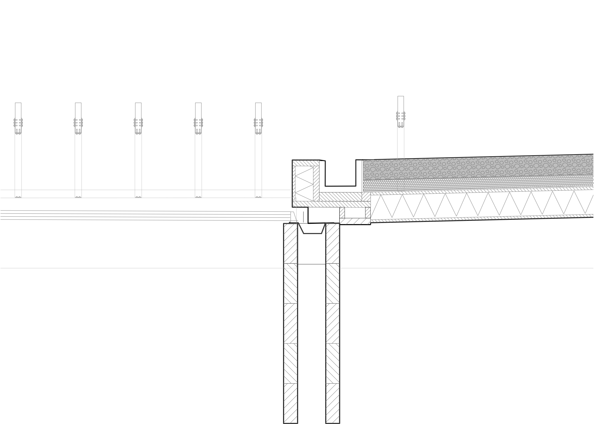
1:10 detail C: connection between glass ceiling & sedem roof
