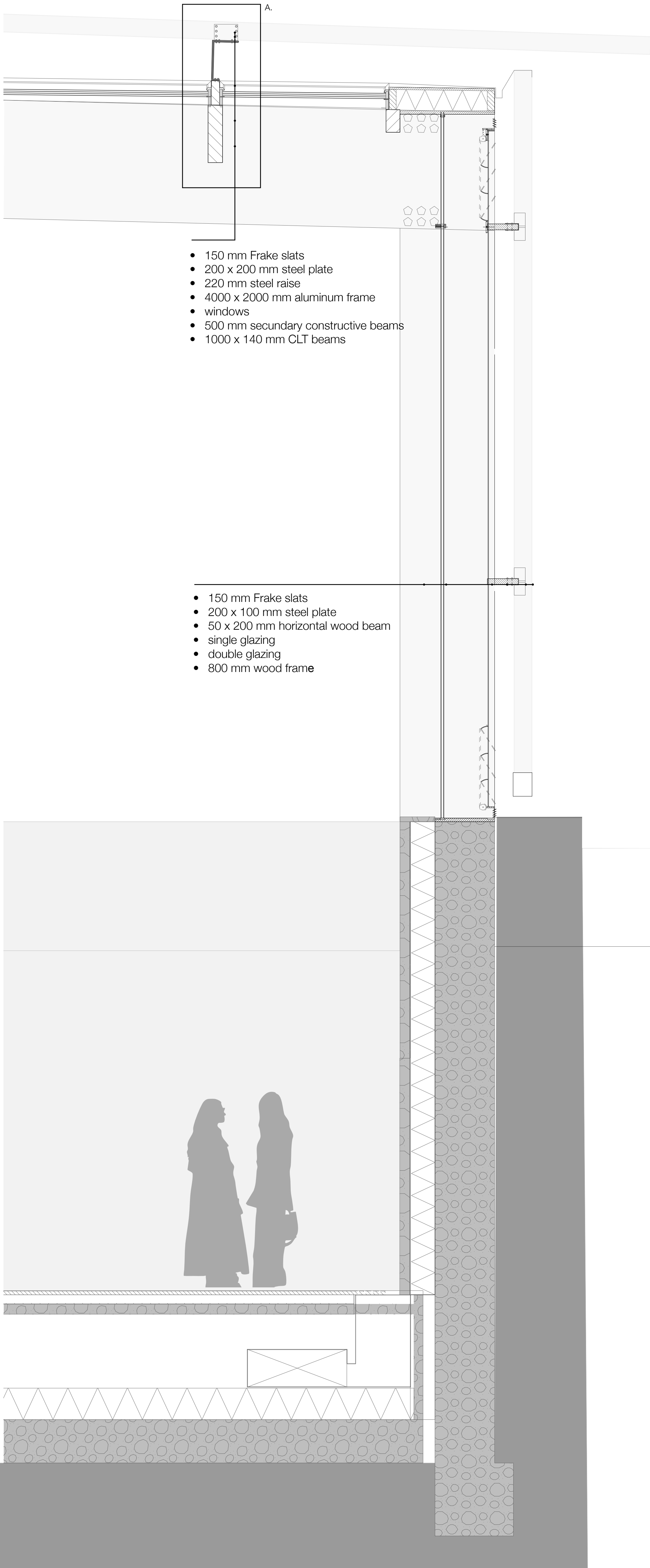
1:20 section south facade glass facade gridline I
