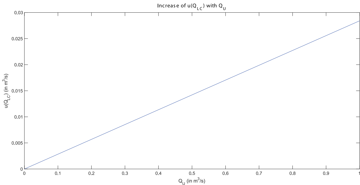
Fig. 13. Example of how the uncertainty u(Q_{LC}) evolves with respect to Q_U . Assumptions done for this plot: T_U = 15\text{ }^{\circ}\text{C} , T_{LC} = 20\text{ }^{\circ}\text{C} , T_D = 16\text{ }^{\circ}\text{C} , u(T_U) = u(T_{LC}) = u(T_D) = 0.05\text{ }^{\circ}\text{C} , u(Q_U) = 0.01 \times Q_U and cov(T_U, T_D) = u(T_U) \times u(T_D) .
