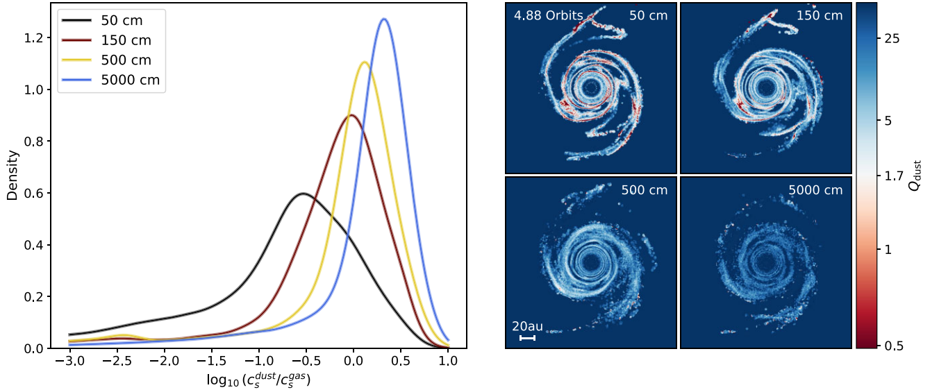
Figure 5. A probability density function (PDF) of the sound speed of dust relative to the gas, c_s^{\text{dust}}/c_s^{\text{gas}} (left-hand panel), for all four dust sizes as described in Fig. 4. The drag force becomes less effective with increasing dust size. Hence, the dust motion becomes uncorrelated with the gas as seen by the increasing velocity dispersion with increasing dust size. The right-hand panels show the Toomre Q of the dust disc for all four dust sizes. The less efficient dust trapping with increasing dust size results in the dust becoming more stable.
