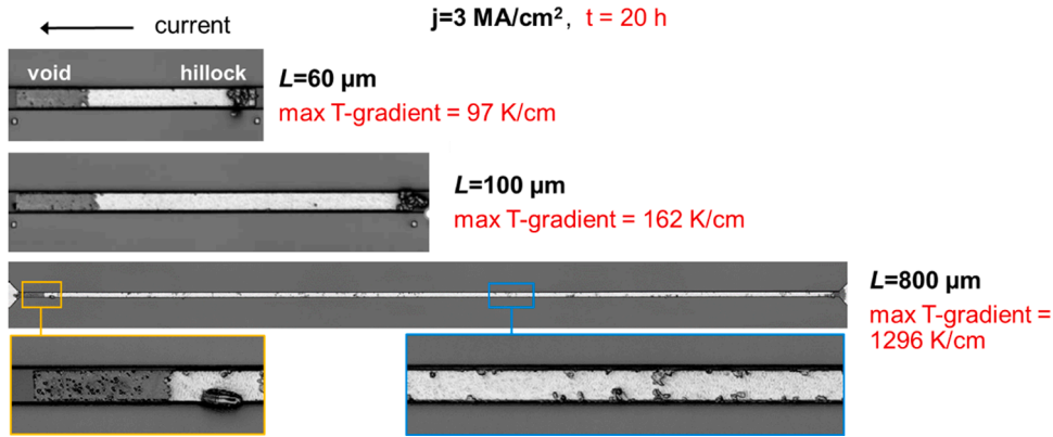
Fig. 3. Optical microscope images for 60/100/800 \mu\text{m} lengths Al lines with Blech structure were under the current density of 3 \text{MA}/\text{cm}^2 and temperature of 250 ^\circ\text{C} at 20 h.
