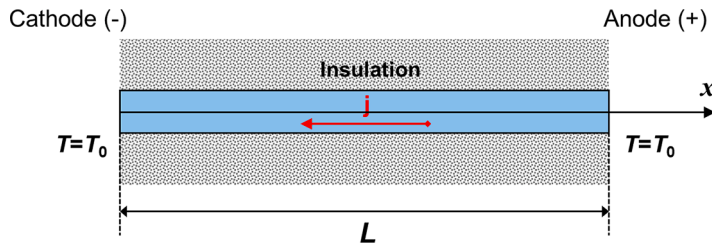
Fig. 7. Schematic of 1D EM problem where atomic concentration C_a(x, t) and hydrostatic stress T(x) are the two unknowns.
