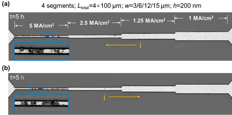
Fig. 5. Optical microscope images of the tapered shape of 400 μm-length Al line. (a) right-to-left current flow (b) left-to-right current flow.
