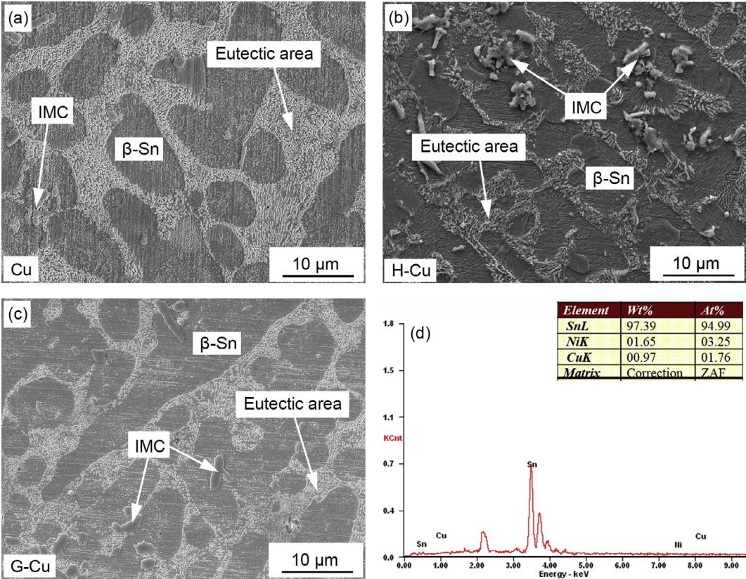
Fig. 5. Microstructure of the solder bulks by SEM: (a) SAC305-0.3Ni on Cu, (b) SAC305-0.3Ni on H-Cu, (c) SAC305-0.3Ni on G-Cu, (d) EDS of \beta -Sn.
