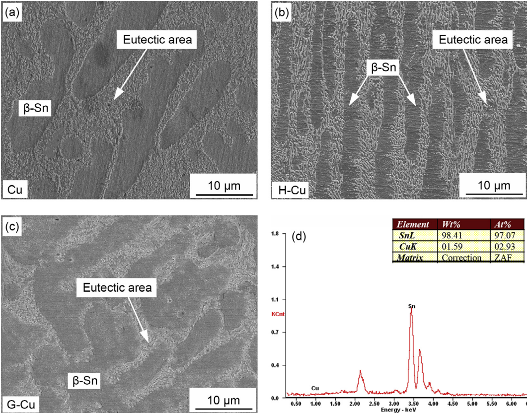
Fig. 4. Microstructure of the solder bulks by SEM: (a) SAC305 on Cu, (b) SAC305 on H-Cu, (c) SAC305 on G-Cu, (d) EDS of \beta -Sn.
