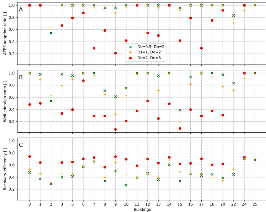
Fig. 13. A: Average ATES adoption ratio ( r_{ATES} ), B: Average well adoption ratio ( r_{wells} ) and recovery efficiency ( \eta_{th} ) of the individual buildings for the most dense ( D_s = 0.5, D_o = 2 ), dense ( D_s = 1, D_o = 2 ) and spacious ( D_s = 2, D_o = 3 ) well placement policies.
