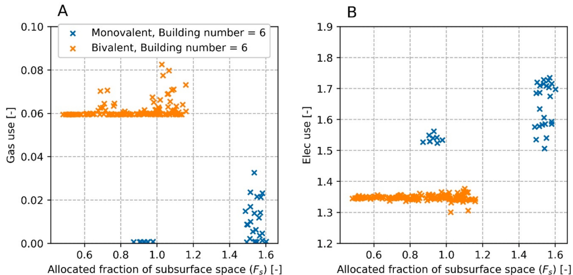
Fig. 20. Relative change in gas (A) and electricity (B) use compared to conventional systems for building 6 with the maximum number of ATEs wells for all mono- and bivalent model realisations. The differences in energy use are therefore only caused by mutual interactions.
