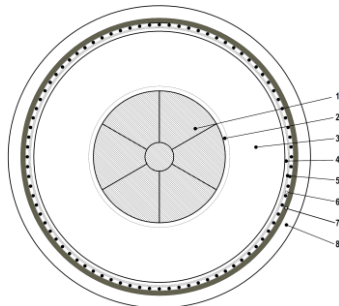
Figure 3. Cross section of the 380 kV cable.
