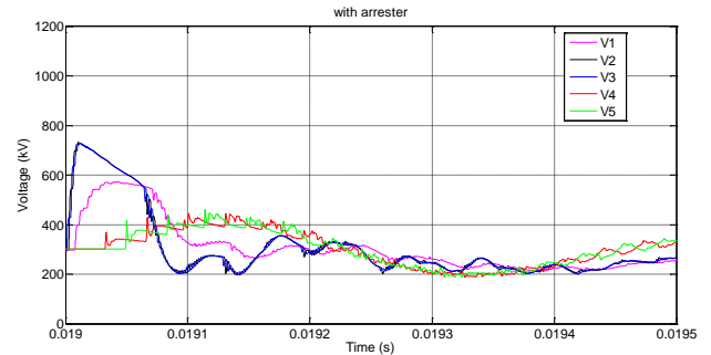
Figure 12b. Voltage responses with arresters for 0.3 km cable.
