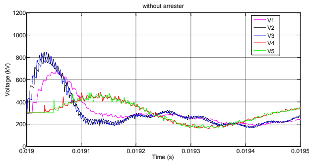
Figure 10a. Voltage responses without arresters for 0.75 km cable.
