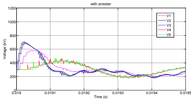
Figure 10b. Voltage responses with arresters for 0.75 km cable.
