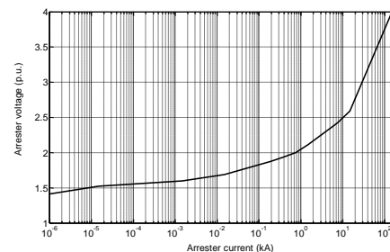
Figure 7. Non-linear v-i characteristic of the applied surge arrester.
