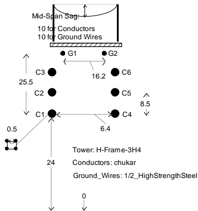
Figure 5. Configuration of the overhead line conductors.
