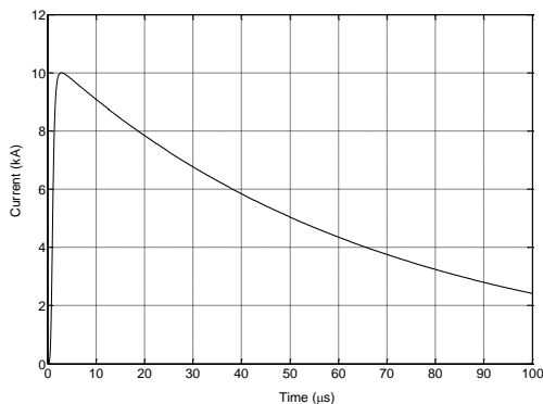
Figure 8. Surge current that is applied to OHL phase conductor.
