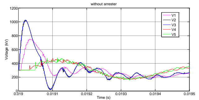
Figure 12a. Voltage responses without arresters for 0.3 km cable.
