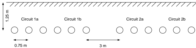
Figure 2. Arrangement of the underground cables.
