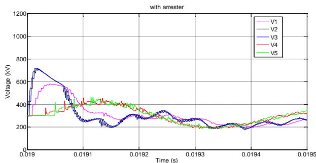
Figure 11b. Voltage responses with arresters for 0.5 km cable.
