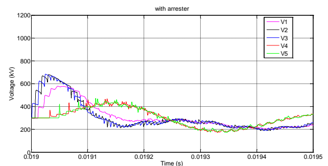
Figure 9b. Voltage responses with arresters for 1 km cable.
