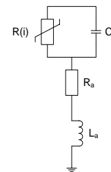
Figure 6. Applied surge arrester model.
