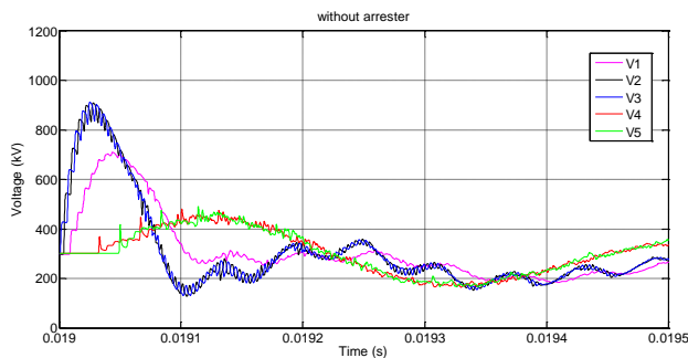
Figure 11a. Voltage responses without arresters for 0.5 km cable.
