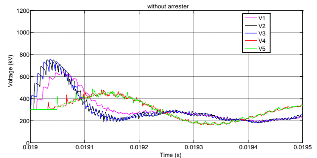
Figure 9a. Voltage responses without arresters for 1 km cable.
