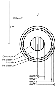
Figure 4. Cross section of the PSCAD cable model of one cable circuit.
