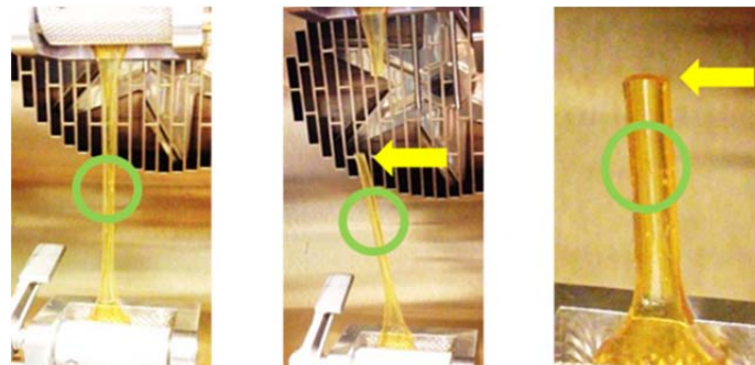
Figure 7. Captures from a video showing the D-1.1 sample breaking away from the healed spot after 30 days of healing at RT. The green circle points out the healed location.
