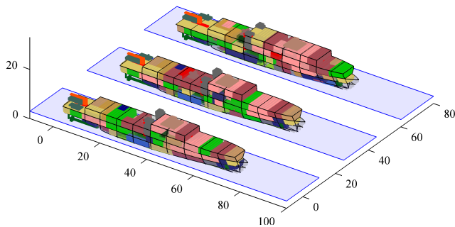
Figure 7.17: Representative design solutions for the hull material choice as highlighted in Figure 7.16. Steel (front), AMS (middle), and GRP (back).
