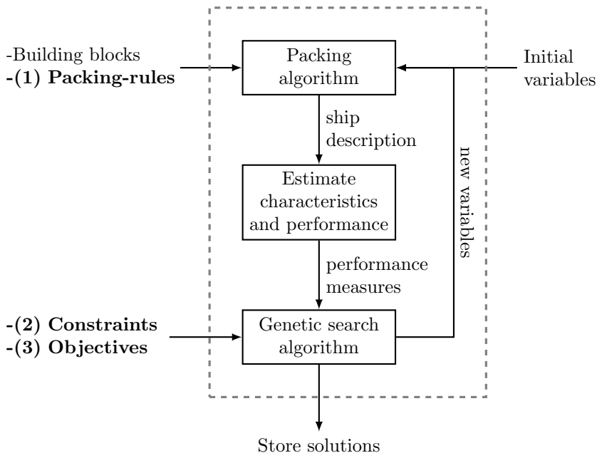
Figure 6.1: Packing-approach process and highlighted inputs that can be used to control the generation of design solutions
