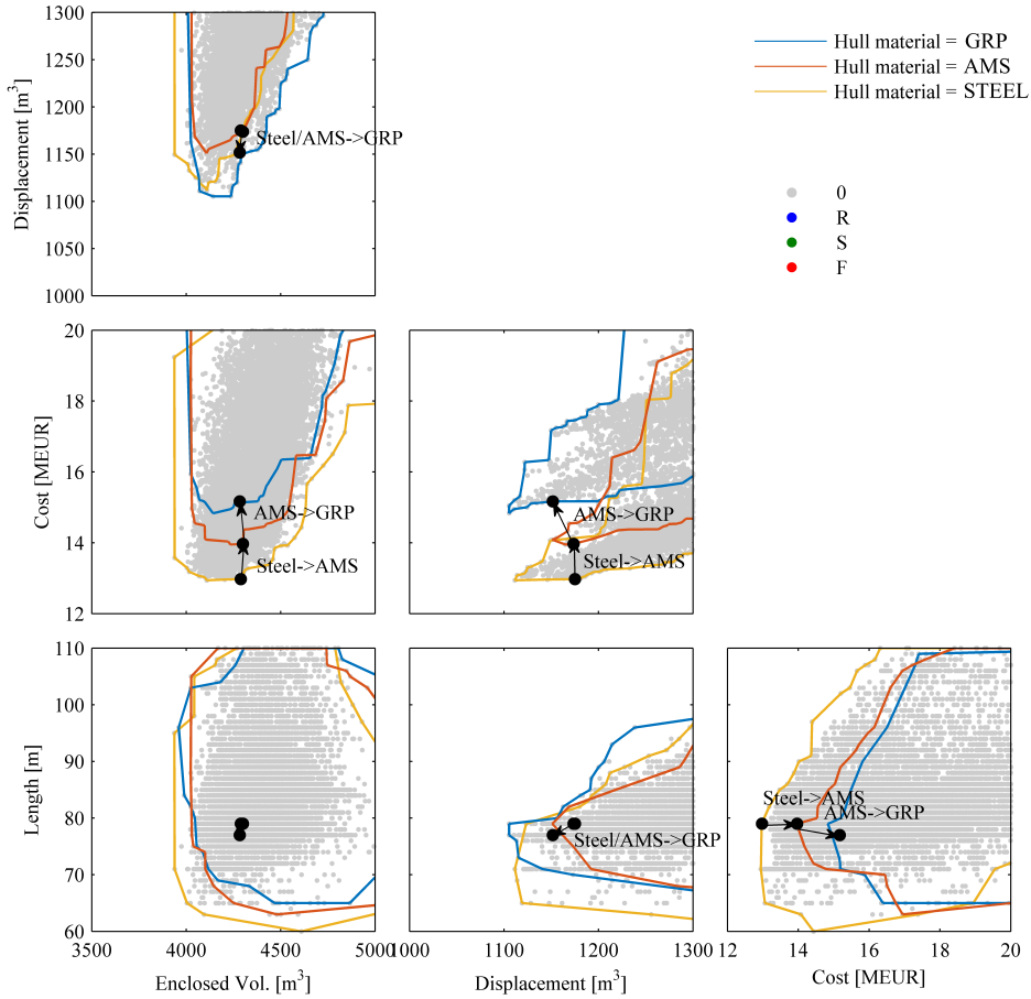
Figure 7.16: Design impact of hull material choice
