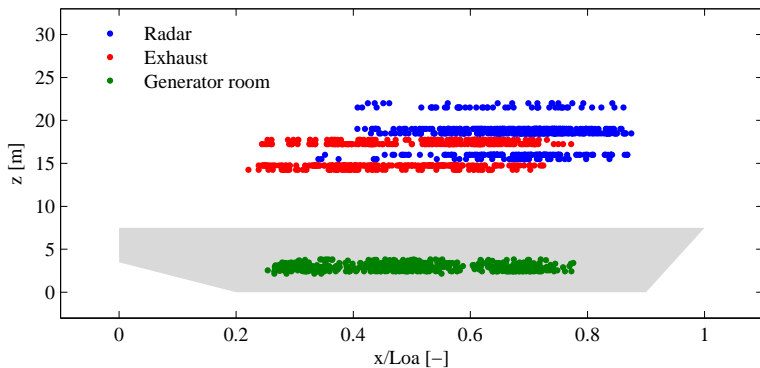
Figure 5.12: Available global positions for multiple systems: radar, exhaust, and generator room.
