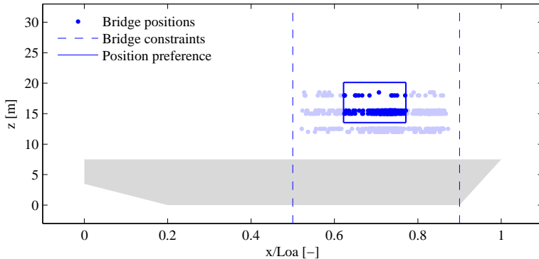
Figure 5.14: Available and preferred global positions for the bridge space after the designer has applied a criterion on the preferred location
