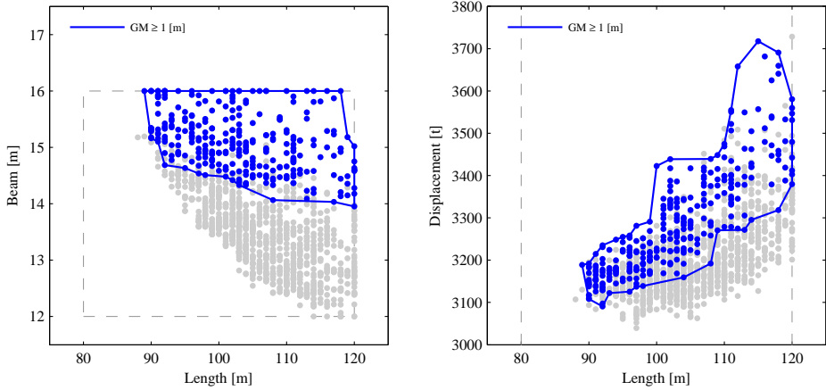
(a) Filtered designs and criterion boundary
