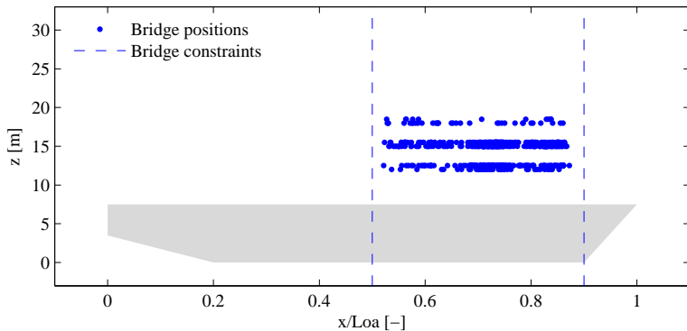
Figure 5.11: Available global positions for the bridge space and its longitudinal positioning bounds
