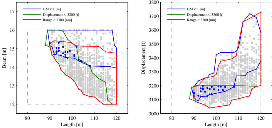
(b) Multiple criteria boundaries
