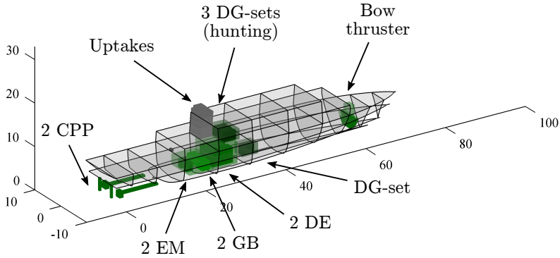
Figure A.3: Example of the modelled propulsion plant in the design of Figure A.1
