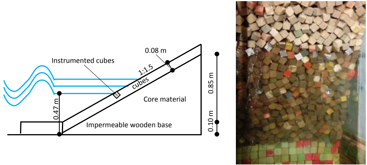
Figure 6. Left: test setup with varying water level. Right: Eight instrumented cubes in model.
