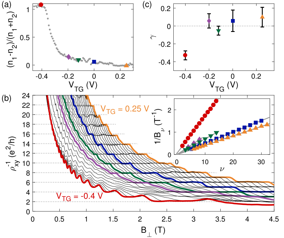
Figure 6.4: (a) Spin-orbit polarization of electron-like states as a function of V_{TG} , with markers defined as in (b). (b) Inverse transverse resistivity, \rho_{xy}^{-1} , for different top gate voltages, V_{TG} . Inset: Inverse magnetic field positions of the filling factors \nu for different V_{TG} values. Solid lines are linear fits to the data. (c) Phase offset \gamma of the data in the inset of (b) extrapolated for 1/B \rightarrow 0 .
