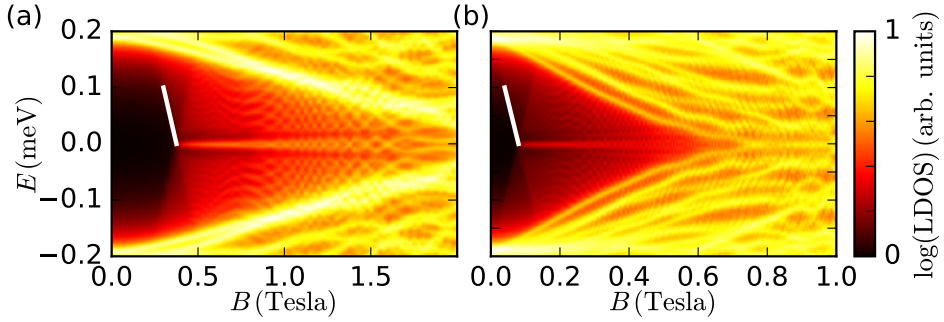
Figure 7.5: (a) (b) show the local density of states (LDOS) at the end of an InAs wire with 40 nm diameter and 2172 nm length in an electric field of \mathcal{E} = 1.2 meV/nm and proximity effect induced superconducting pairing \Delta = 0.2 meV. The chemical potential \mu = 39.6 meV ( \mu = 68.5 meV) is tuned to the |l| = 1 ( |l| = 2 ) subbands. The slope of the whites lines amount to a g -factor of 23 (43).
