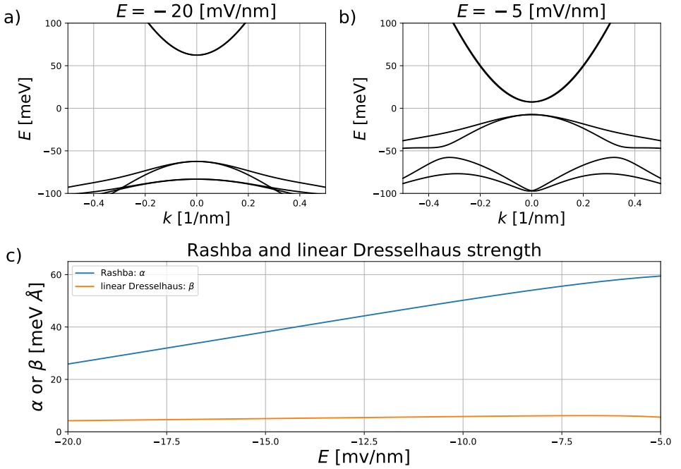
Figure 5.3: Numerical calculation of the spin-orbit interaction in InAs/GaSb quantum well. Applied electric field tunes system into the single-carrier regime (non inverted band structure). (a, b) Band structure along the [100] direction. (c) Strength of the Spin-orbit interaction in function of applied electric field. Rashba coefficient \alpha (blue) reacts strongly to applied electric field, whereas effect on linear Dresselhaus coefficient \beta (yellow) is almost neglectable.
