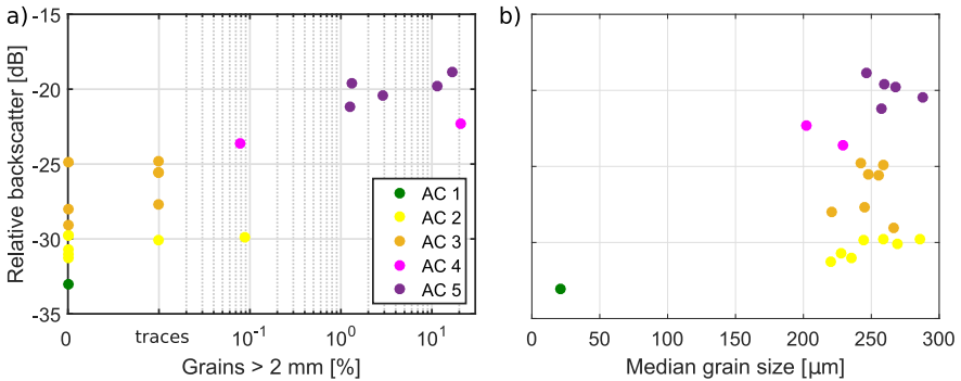
Figure 4.8: Comparison of acoustic data (05/18) with box core samples (05/18). a) BS vs. percentage of grains larger than 2 mm. b) BS vs. median grain size, d_{50} value, of the sand and mud fraction.
