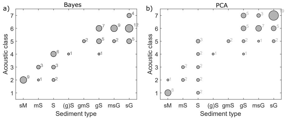
Figure 3.10: Correlation between AC and sediment type at grab sample locations. a) Bayesian method, b) PCA. Dots indicate the number of matches between AC and sediment type. The sediment type is determined after Folk [83].
