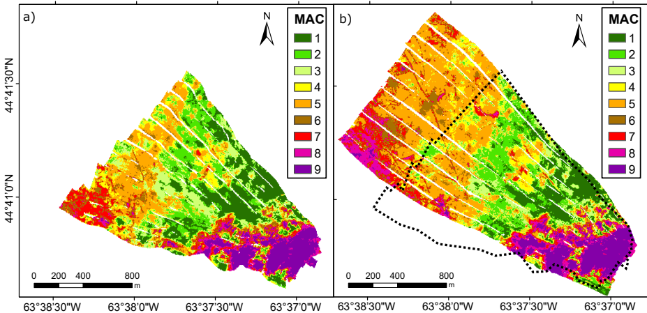
Figure 5.13: MAC map of the Bedford Basin in a) 2016 and b) 2017 obtained from the combination of the individual single frequency maps. The spatial resolution is 5 m by 5 m.
