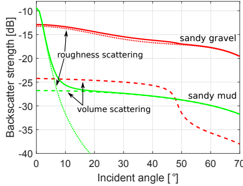
Figure 2.5: APL-model: Backscatter strength at 90 kHz for representative sandy mud and sandy gravel seabed. Individual contribution of roughness and volume scattering are shown as well. Same geoacoustic parameters as used in Fig. 2.2 are employed. In addition, sandy mud: \gamma = 3.25 , \eta = 5.17 \times 10^{-4} \text{ cm}^4 , \hat{\sigma}_v = 0.001 ; sandy gravel: \gamma = 3.5 , \eta = 2.19 \times 10^{-2} \text{ cm}^4 , \hat{\sigma}_v = 0.002 are used (see also Appendix B.1).
