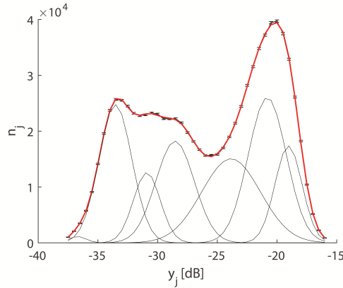
Figure 3.3: Shown here is the histogram of the measured BS data n_j per 0.5 dB bin y_j from the data collected in 2014 and 2015 (black line with error bars) which is almost hidden by the modeled f(y_j | x) in red. Also displayed are the 7 Gaussians in black.
