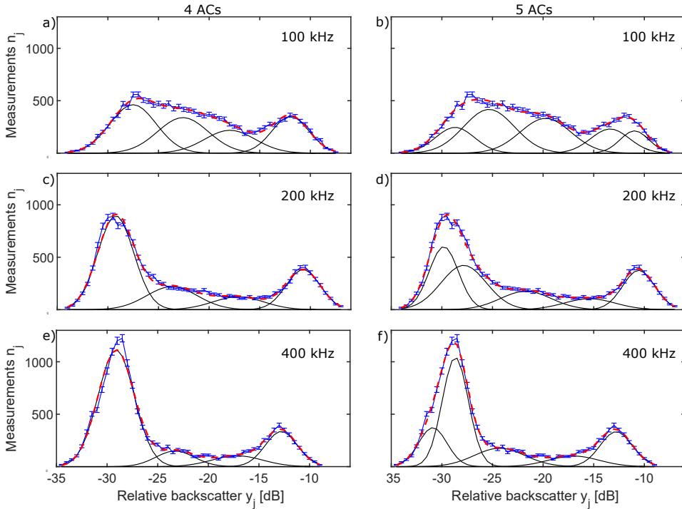
Figure 5.7: Model fits to the histogram of the measured BS data n_j (blue) per 0.5 dB bin y_j at a,b) 100, c,d) 200, and e,f) 400 kHz are displayed. The measured BS data are obtained from the 54^\circ incident angle of the starboard side from the Bedford Basin 2016 dataset. The blue error bars indicate the variance of the measurements per bin. The modeled f(y_j|\mathbf{x}) histogram calculated by using a,c,e) 4 Gaussian distributions and b,d,f) 5 Gaussian distributions is shown in red. The corresponding Gaussians are displayed in black.
