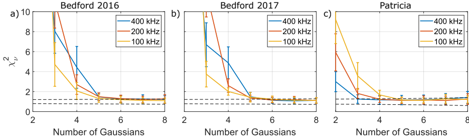
Figure 5.6: Chi-square test applied to the a) Bedford 2016, b) Bedford 2017, and c) Patricia Bay dataset for incident angles from 40^\circ to 60^\circ of the starboard and port side. The solid lines and their error bars represent the mean and standard deviation of the \chi^2_v values of all considered angles. The black dashed lines show the \chi^2_v value of 1 \pm \sqrt{2/v} , which indicates a good model fit (see Section 3.3.2).
