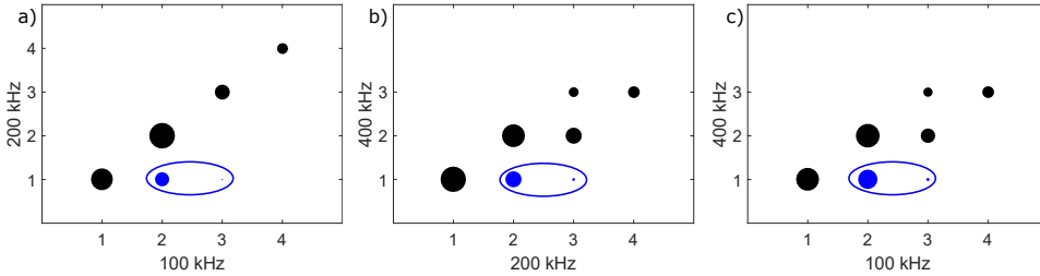
Figure 5.11: Matching matrix between the ACs of a) 100 and 200, b) 200 and 400, and c) 100 and 400 kHz for the Patricia Bay.
