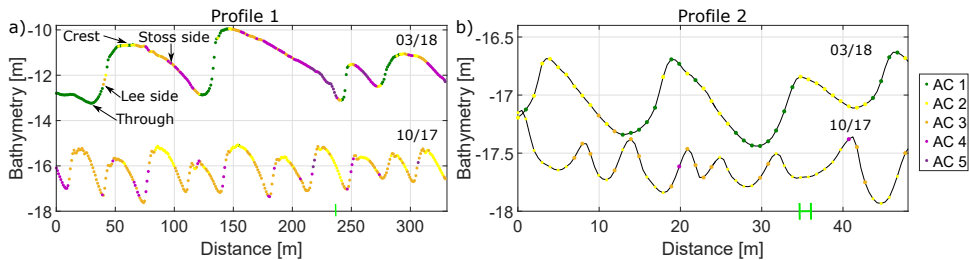
Figure 4.12: Bathymetric and ASC cross-profiles for Profile 1 and 2 of the October 2017 and March 2018 measurements. Location of Profile 1 and 2 are indicated Fig. 4.11. Green bar at the x-axis indicates resolution of the slope calculation.
