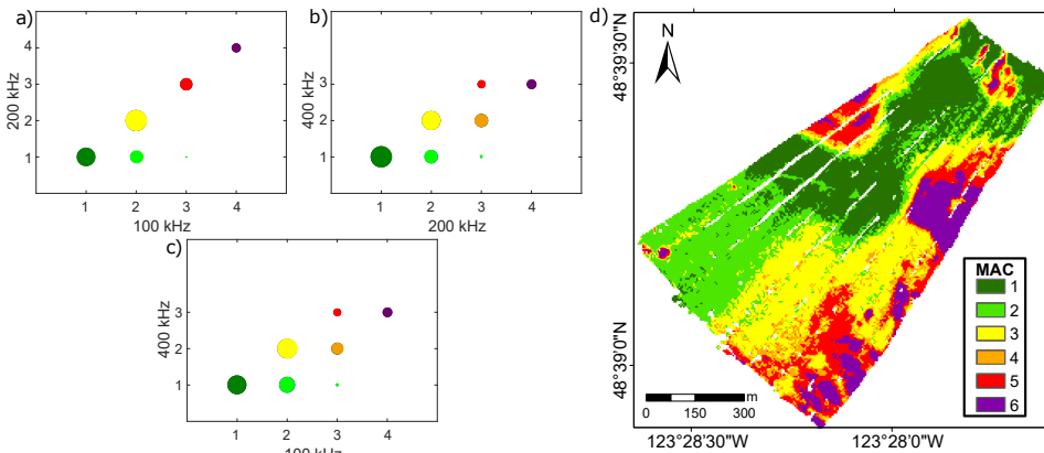
Figure 5.14: Multispectral classification results of the Patricia Bay dataset. MAC revealed by the AC combinations of a) 100 and 200, b) 200 and 400, and c) 100 and 400 kHz. The colors indicate the different MACs. d) MAC map with spatial resolution of 5 m by 5 m.
