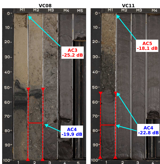
Figure 4.15: Depth profile of vibrocores VC08 and VC11 located in the tidal-channel in May 2018. Red horizontal bar indicates location of surficial seabed from April 2017 measurement (before nourishments). Error bars indicate maximum depth variation within a radius of 5 m around the sample location. Blue and red font indicate AC and BS value at the sample location for April 2017 and May 2018 measurements, respectively.
