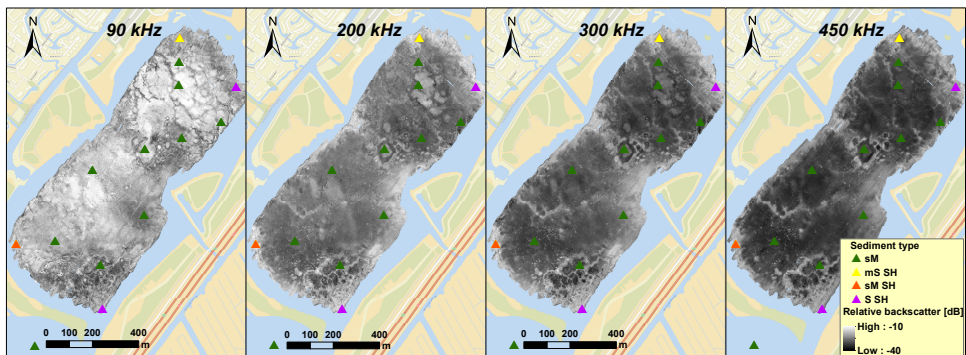
Figure 6.4: BS mosaics measured in the Vlietland Lake at 90, 200, 300, and 450 kHz. The grid cell size is 1 m by 1 m. Abbreviations: sandy mud (sM), sandy mud with shells (sM SH), muddy sand with shells (mS SH), and sand with shells (S SH).
