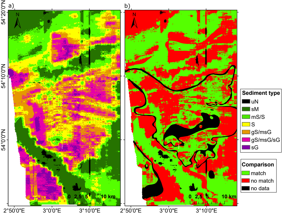
Figure 7.9: a) Full-coverage sediment map (ASC map) based on interpolated AC map (Fig. 7.6a) and 46 grab samples (Table 7.3). b) Map comparison between full-coverage sediment map (Fig. 7.9a) and the existing EMODnet seabed sediment map (Fig. 7.1b). "No data" implies either the Folk sediment type is not available in one of the maps or an AC is unassigned in the interpolated ASC map.
