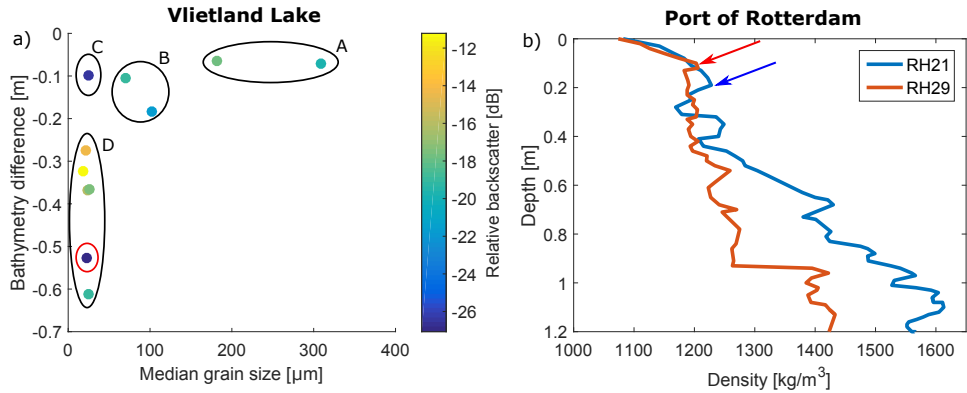
Figure 6.8: a) Measured depth difference between 90 and 450 kHz versus median grain size at all sample locations (Fig. 6.1c) in the Vlietland Lake. The colorbar indicates the averaged BS level (BS mosaics) at 90 kHz around the sample locations. The subsets, denoted A, B, C, and D are defined based on the sediment properties, BS level and the measured bathymetry difference at the sample location. b) Density profiles at two locations taken with a rheometric profiler in the Port of Rotterdam (Fig. 6.1d).
