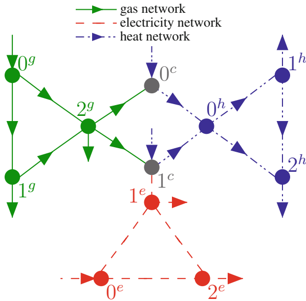
Fig. 1 Network representation of a small MES. Each SCN consists of three nodes. The gas and electricity networks have an external source connected at nodes 0^g and 0^e , the heat network has no external sources. In each SCN, nodes 1 and 2 are sinks. The SCNs are coupled by a gas-boiler, node 0^c , and a combined heat and power plant (CHP), node 1^c . The links show defined direction of flow, the terminal links show actual direction of flow
