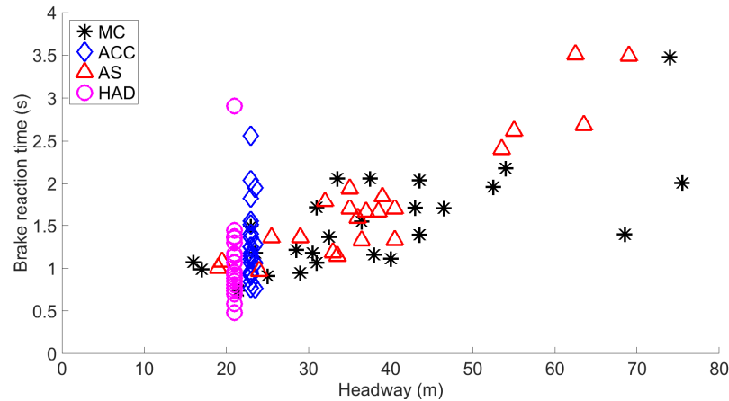
Figure 6 Brake reaction time vs. headway at the moment the lead car started to decelerate (Experiment 2). MC = manual control ( N = 26 ), ACC = adaptive cruise control ( N = 26 ), AS = automated steering ( N = 22 ), HAD = highly automated driving ( N = 27 ) (see online version for colours)
