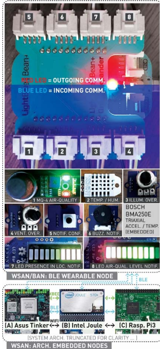
Figure 2. BLE Wearable Node as WSN / BAN, Features.
