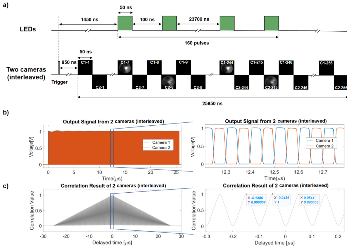
Fig. 4. 20 Mfps interleaved imaging results of strobe LEDs. (a) The timelines of the LEDs and the two cameras with selected frames of recorded imaging LEDs. Each green box represents when the LEDs were emitting during the interleaved imaging of the two cameras. C1 and C2 represent camera 1 and camera 2, respectively, and the number after the dash is the frame number. See the complete recording in Video S1 (online only). (b) Output signals of the exposure timing of each recorded frame from two cameras (c) Cross-correlation of the two signals of exposure timing. LEDs = light-emitting diodes.
