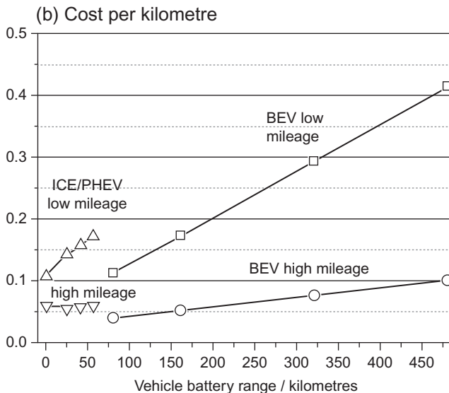
Fig. 2 Cost per kilometer ($/km) for hybrid cars (Internal Combustion Engine combined with a Plug-in Electric motor, ICE/PHEV) and for BEVs. “Low” yearly mileage of 13,216 km is compared to a vehicle utilization rate increased by 5 times to a “high” yearly mileage of 66,064 km ( Offer, 2015 ).
