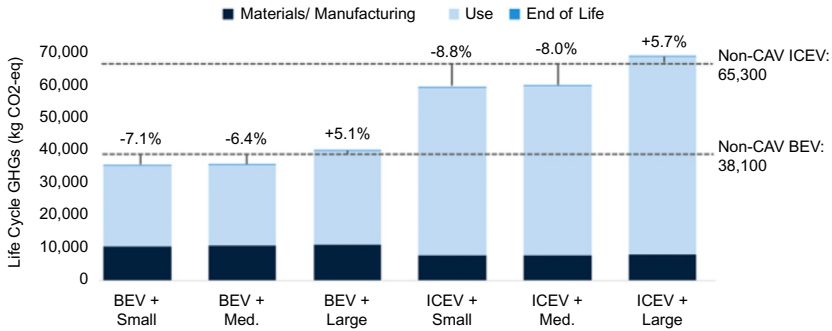
Fig. 1 Life cycle greenhouse gas emissions (GHGs) for six highly automated vehicles. (Gawron et al., 2018).
