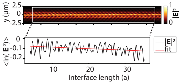
Figure 6.4: (a) Normalized ensemble-averaged electromagnetic field intensity map, averaged over 5 realizations of bearded interface without intentionally induced disorder of the non-trivial mode with integrated over fast light region. Inset: Ensemble-averaged field intensity profile fitted with a linear slope to obtain the backscattering mean free path.
