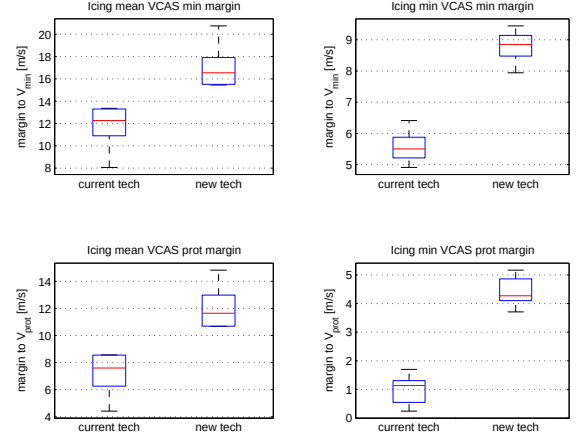
Figure 21. Statistical analysis of angle of attack and speed margins to envelope boundaries for icing scenario, all pilots
