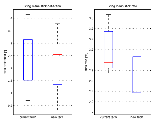
Figure 23. Statistical analysis of pilot activity for icing scenario, all crews
