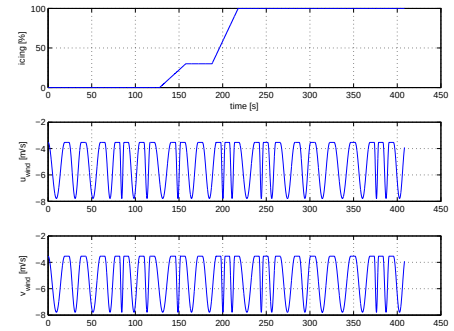
Figure 15. Icing progress and wind gust conditions
