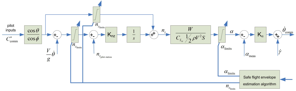
Figure 4. Longitudinal control law setup with adaptive envelope limits
