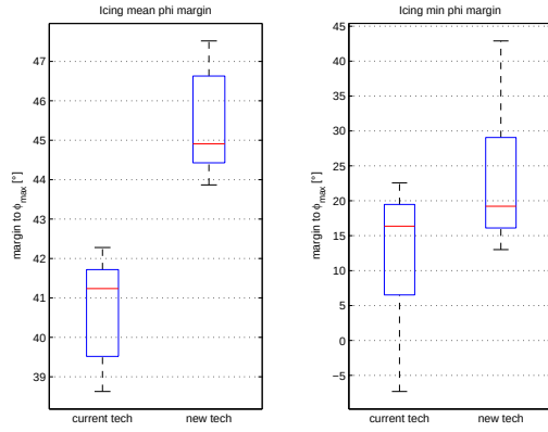
Figure 22. Statistical analysis of bank angle margin to envelope boundaries for icing scenario, all crews
