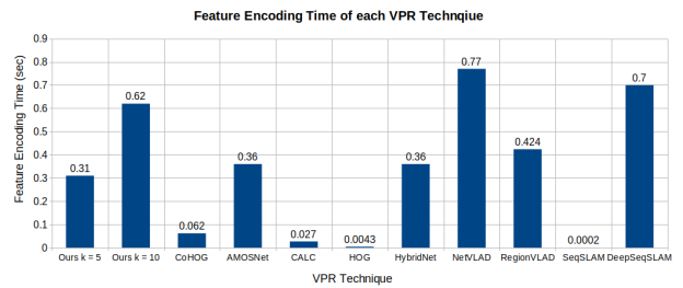
FIGURE 4. The feature encoding time of various VPR technique are presented in this graph. Our k=5 and k=10 represent the feature encoding time of ConvSequential-SLAM using fixed sequences of 5 and 10 images respectively.
