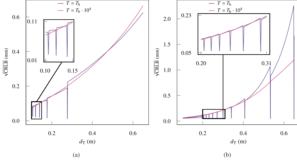
Fig. 8. CRLB calculated for two reflectivity conditions and two different T values. The system parameters are P_s = 7.36 mW, N_{\text{TCSPC}} = 30000 , \Delta_{\text{TDC}} = 25 ps, and E_n = 0.4 \text{ W m}^{-2} \text{ nm}^{-1} . In (a) \rho is 8 % and in (b) \rho is 60 %.
