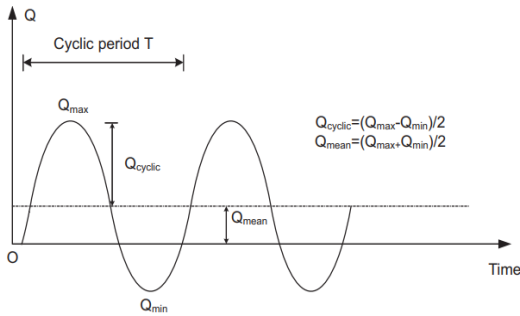
Figure 1 Cyclic loading nomenclature (Tsuha et al., 2012).
