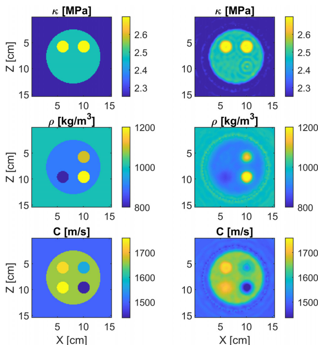
FIG. 15. (Color online) Medical ultrasound inversion results obtained using the CG method.
