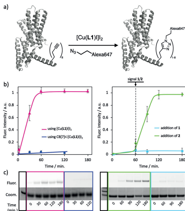
Figure 3. a) [\text{Cu}(\text{L1})]\text{I}_2 -catalyzed fluorescence labeling of alkyne-handle-modified vinculin protein with azide-Alexa 647. The recombinant vinculin protein has eight alkyne groups at various positions in its structure. b) Left: Relative conversion of fluorescence labeling over time. Uninhibited fluorescence labeling reached its maximum value after approximately 60 min (magenta), whereas no significant conversion was observed for CB[7]-inhibited fluorescence labeling over the course of 120 min (blue). Right: Activation of fluorescence labeling using signal molecules. No catalyst activation was observed when signal molecule 1 was added after 60 min (dashed line) to a sample with the CB[7]-inhibited catalyst (cyan). In a similarly inhibited sample, the addition of signal molecule 2 after 60 min led to immediate fluorescence labeling (green). Lines have been drawn to guide the eye. c) Scans of gels stained with Coomassie (Coom.) and analyzed for fluorescence intensity (Fluor.) over time (min). Coomassie bands shown in the black frames indicate the 40 kDa protein marker (recombinant vinculin MW is 35.6 kDa (453–724 amino acid sequence of wild-type vinculin)).
