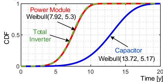
Fig. 6. Wear-out failure Cumulative Distribution Function (CDF) of power modules and capacitor bank.
