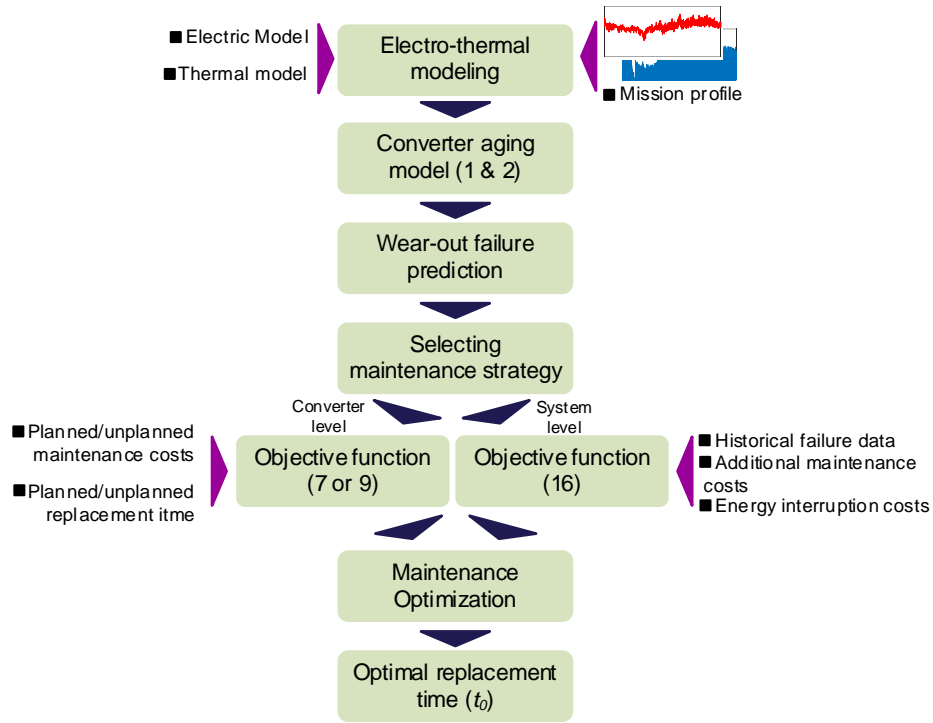
Fig. 3. Proposed maintenance scheduling process in power electronic converters.
