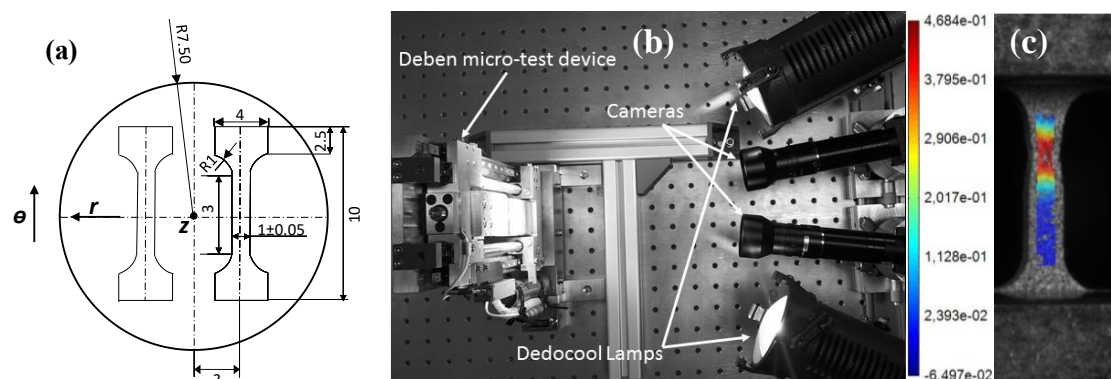
Figure 1. (a) Tensile sample extraction scheme with simple shear geometry, (b) tensile test and camera setup during an experiment and (c) full-field strain map using 3-dimensional digital image correlation (3D DIC).
