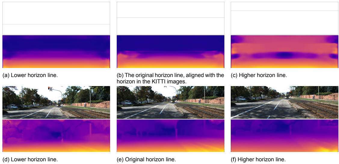
Figure 3.5: a-c : The vertical position of the horizon line does not change the ground plane. While it has some influence on the depth map, the ground plane still seems to end at the same height in the image. d-f : In real images, the extent of the ground plane matches the position of the horizon. This suggests that MonoDepth has a mechanism to detect the horizon that is not triggered in images a-c ; it is not yet understood how this works. Input images d-f : KITTI stereo vision dataset (CC BY-NC-SA 3.0)
