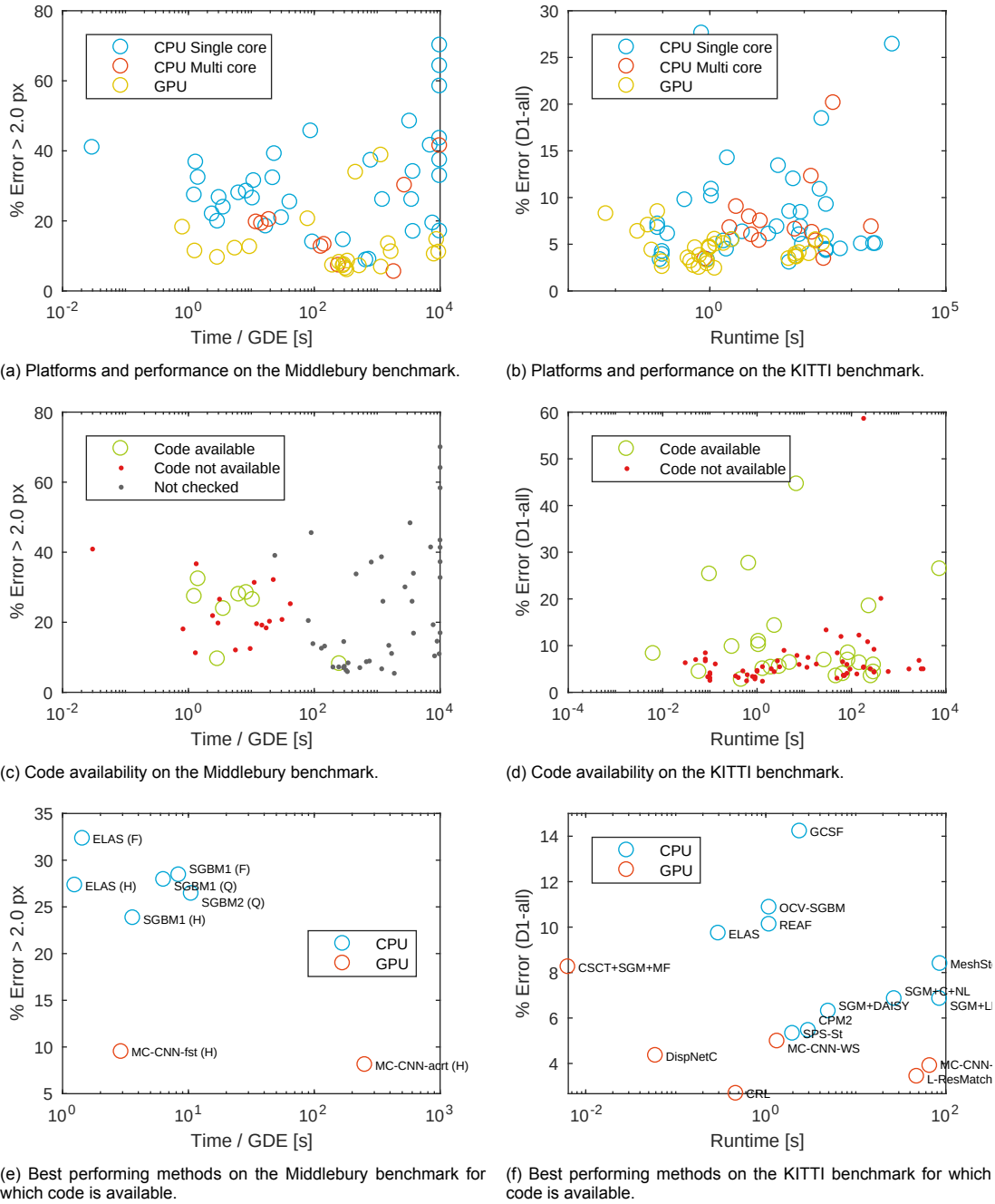
Figure 2.3: Scatterplots of accuracy versus runtime performance on the Middlebury 1 and KITTI 2 stereo vision benchmarks. Runtime on the Middlebury benchmark is measured in seconds per Giga Disparity Evaluations (GDE), which is found by multiplying the image width, height and maximum number of disparities. Data obtained on 27/11/2017. a, b : Methods running on the GPU tend to perform better than those running on the CPU. On the Middlebury benchmark they perform better in terms of accuracy, while on the KITTI benchmark they also outperform CPU methods in terms of runtime – perhaps because runtime performance is more important for automotive applications than for the static pictures of Middlebury. c, d : While code is not available for every method, there are enough close-to-optimal algorithms for which source code has been published. e, f : These methods should be considered first when choosing a stereo vision algorithm, as they perform well and their code is publicly available. Popular choices are ELAS [17] and SGM/SGBM [22]; the latter is also included in OpenCV.
