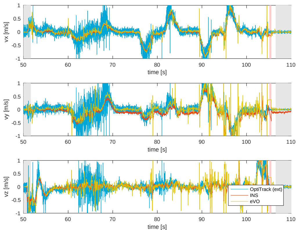
Figure 3.11: Body-frame velocities estimated using embedded Visual Odometry (eVO) compared to the ground-truth from OptiTrack. The figure shows both the raw estimates (eVO) and the velocity estimates after fusion with the accelerometer readings (INS). In general the estimate of eVO corresponds well to the OptiTrack measurements and appears to be less noisy (this may depend on the OptiTrack calibration and lighting conditions in the Cyberzoo ). The INS estimates have a slight bias (especially in the y axis) that comes from the accelerometer. Possibly the SLAMDunk is not placed exactly above the Center-of-Gravity (CoG) of the drone.
