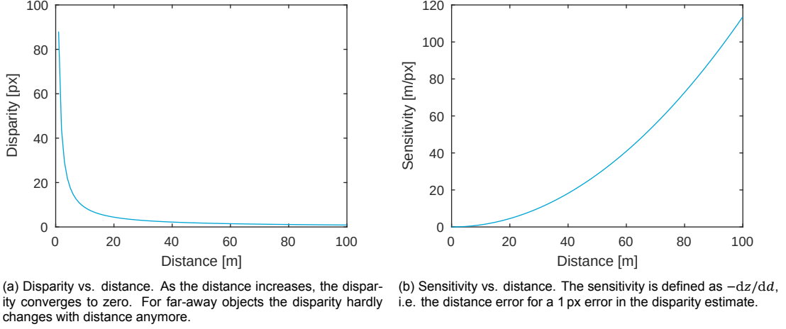
Figure 2.4: Maximum range of stereo vision. As the distance increases, the sensitivity to stereo matching errors increases quadratically. Example plots generated for a camera with baseline B = 20 cm and focal length f = 400 px. Best-case disparity errors are in the order of 0.5 px to 0.1 px [43] depending on the algorithm.
