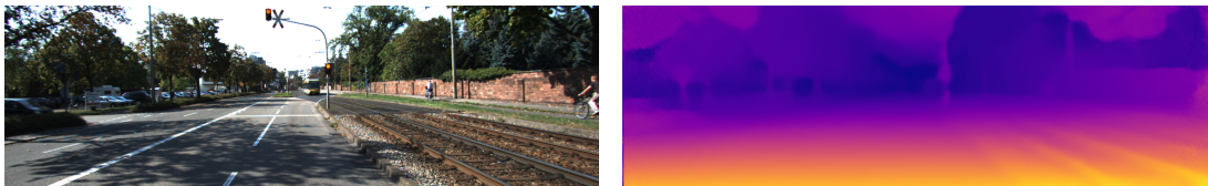
Figure 3.1: Monocular depth estimation with MonoDepth [20]. Input image: KITTI stereo vision dataset (CC BY-NC-SA 3.0)
