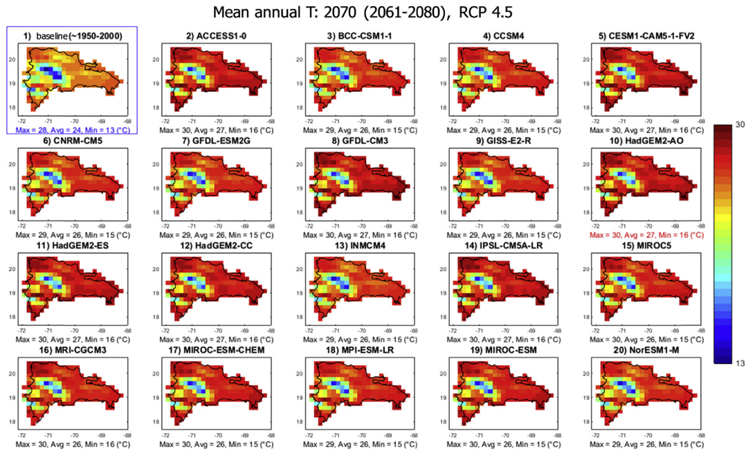
FIGURE 3.7 Spatial distribution of mean annual T ( ^{\circ}\text{C} ) over Dominican Republic for the period 2061–80 (2070): baseline and 19 GCMs, and RCP 4.5. GCM, General Circulation Model; RCP, Representative Concentration Pathway; T , temperature.
