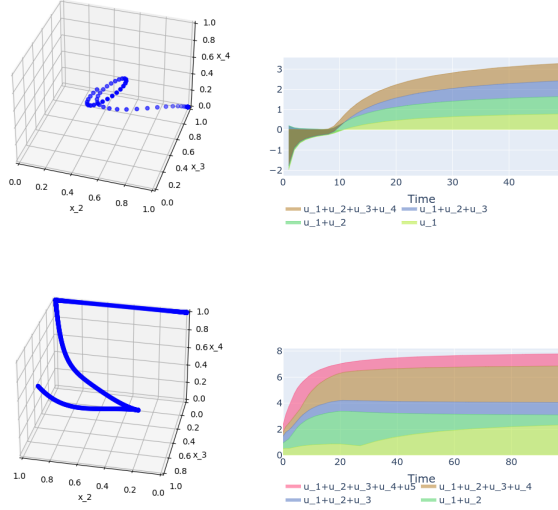
Figure 3: Time-average payoffs and social welfare of a sample learning trajectory in the matched-mismatched pennies game (top), and in the asymmetric 5-penny game with p = 3 (bottom, projection onto first three variables).
