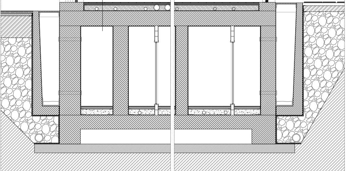
Detail 4 - Foundation and storage
