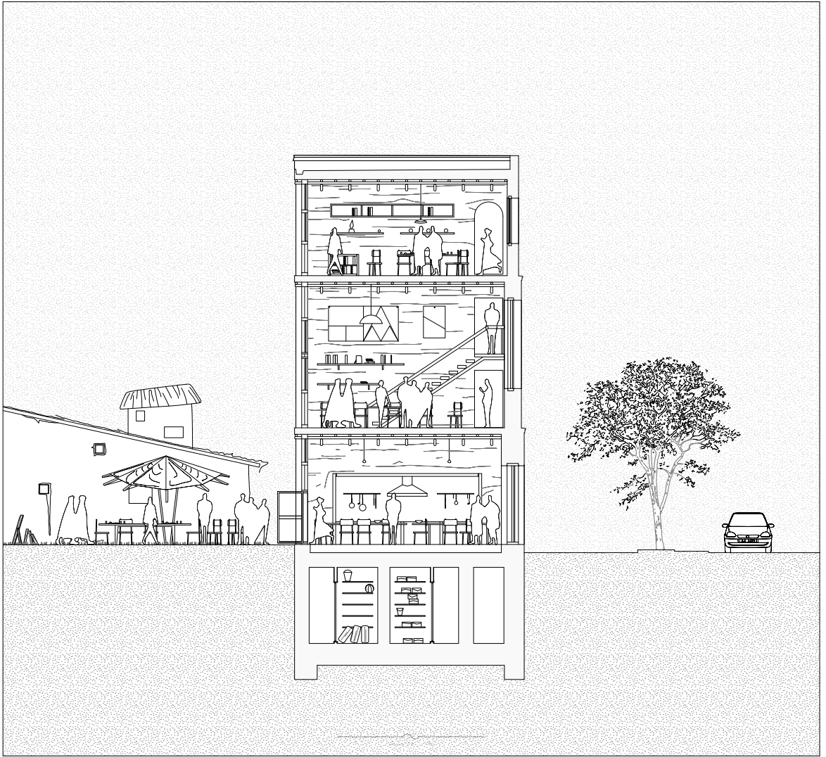
Transversal section #1
