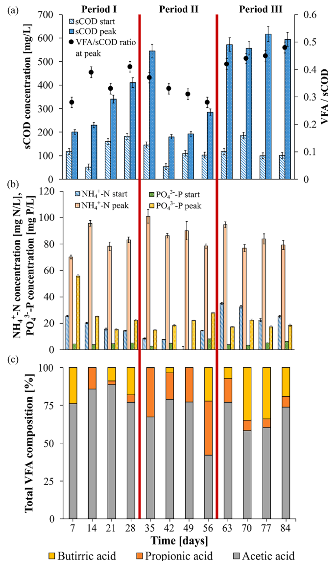
Fig. 2. VFA and sCOD production (a), ammonium and phosphate release (b) and VFA composition (c) obtained during the fermentation.
