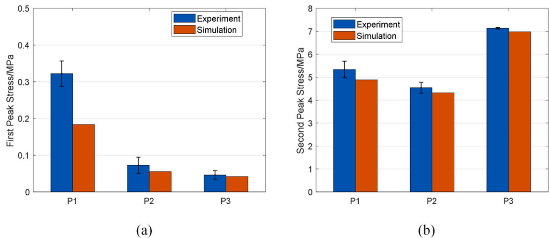
Fig. 13. Comparison of a) the first peak stress, (b) the second peak stress.
