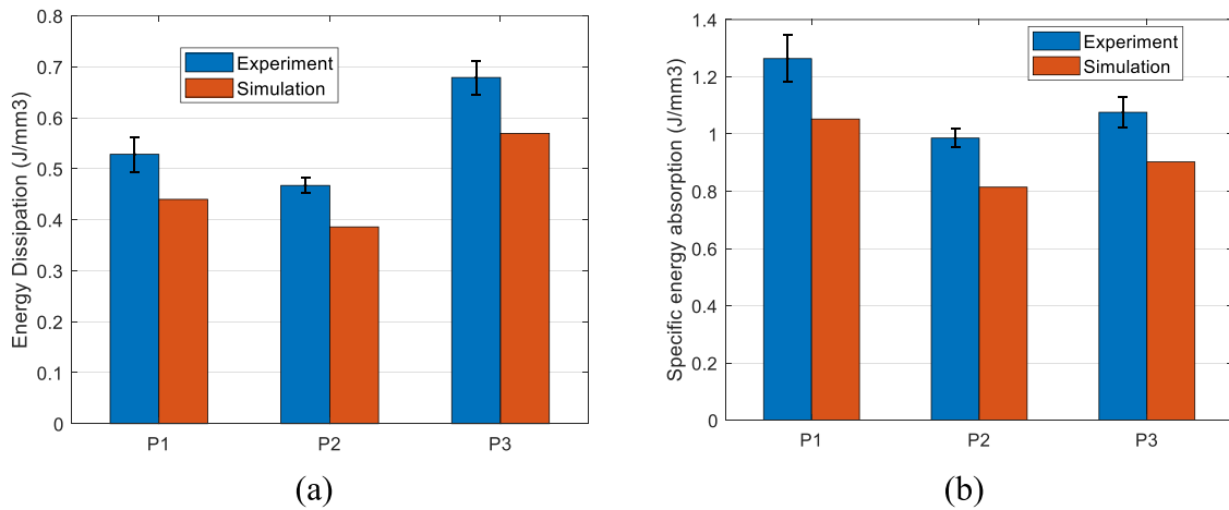
Fig. 16. Comparison of the energy dissipation until the second peak stress, (a) energy dissipation by integrating the stress-strain curve, (b) specific energy absorption.
