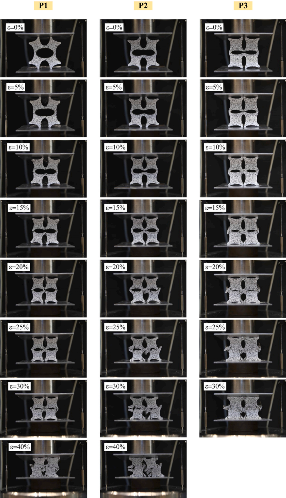
Fig. 11. The deformation process of ACCCs under compression.
