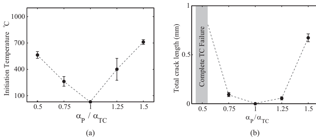
Fig. 6. Variation of (a) crack initiation temperature and (b) total crack length for different CTE mismatch ratios \alpha_P / \alpha_{TC} = 1.5, 1.25, 1, 0.75 and 0.5 . For the CTE mismatch ratio of 0.5 , there is a complete failure of the TC before reaching the final temperature ( 30^\circ\text{C} ) as indicated by a grey shade.
