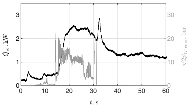
b) Heat flow into the acoustic pressure sensor water cooling
