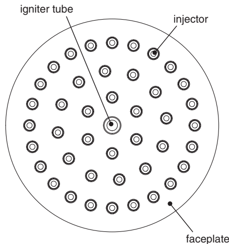
Fig. 2 Injector pattern of BKD [25].
