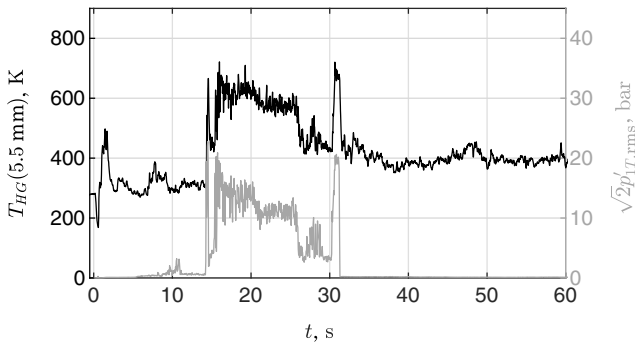
a) Hot gas temperature at 5.5 mm downstream the injection plane
