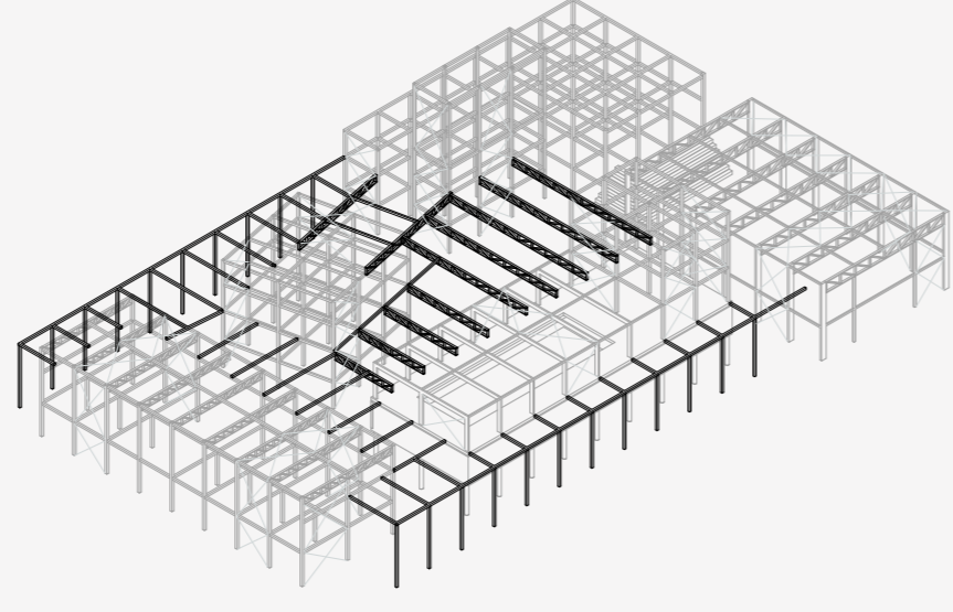
2. In between the volumes, the roof structure is places and connected to the volumes themselves.
