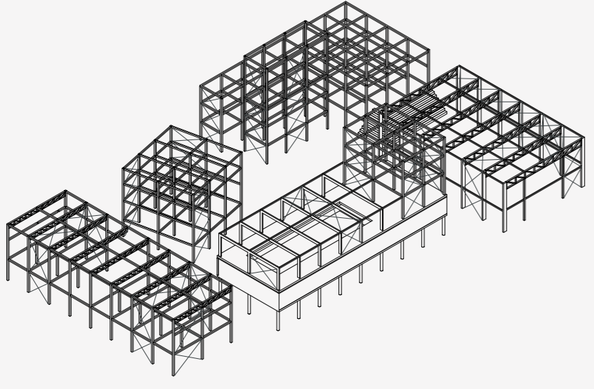
1. All volumes consist out of steel columns and beam construction, the structure stability is facilitates with cross-beams
