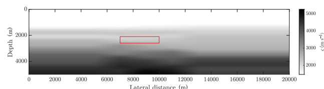
Figure 10. The smooth velocity model provided by Equinor for migration. The red rectangle inside the velocity model indicates the second target area, and the virtual source and receiver positions are at the upper boundary.
