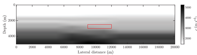
Figure 5. The smooth velocity model provided by Equinor for migration. The red rectangle inside the velocity model indicates the first target area. The virtual source and receiver positions are at the upper boundary of this target area.
