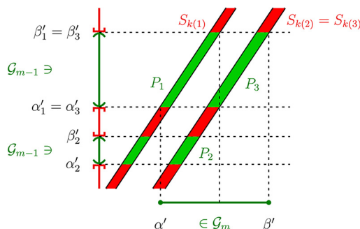
Fig. 8. The definition of the parallelograms P_j .
