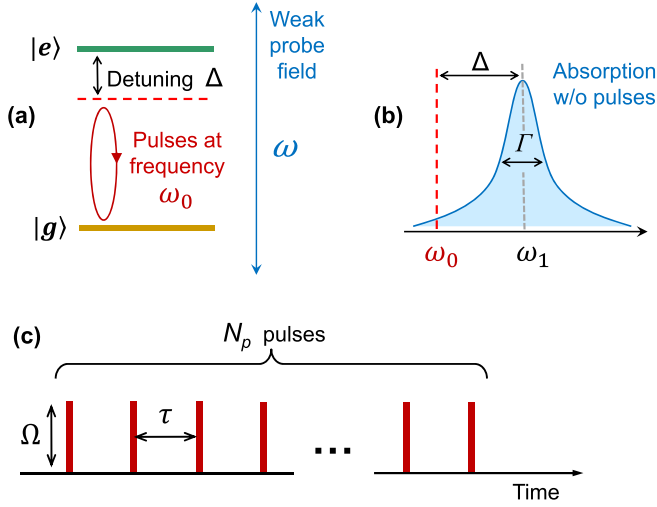
FIG. 1. (a) Schematic representation of the two-level system with ground state |g\rangle and excited state |e\rangle separated in the rotating frame by the detuning \Delta . It is probed by measuring the energy absorbed from a weak field as a function of frequency. (b) The absorption spectrum in the absence of any driving field has a Lorentzian line shape centered around \Delta . (c) We will evaluate the absorption spectrum when the system is driven by a periodic sequence of \pi pulses with interpulse time \tau .
