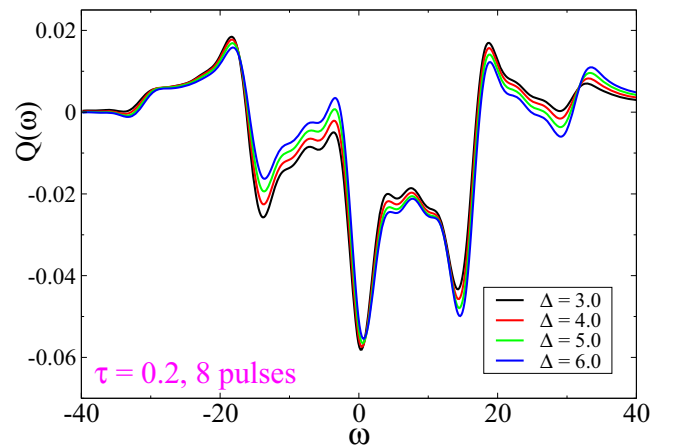
FIG. 5. Absorption spectrum of the TLS with detunings \Delta = 3.0 (black), \Delta = 4.0 (red), \Delta = 5.0 (green), and \Delta = 6.0 (blue) driven by a periodic sequence of \pi pulses of period \tau = 0.2 after N_p = 8 pulses. The curves present analytical results.
