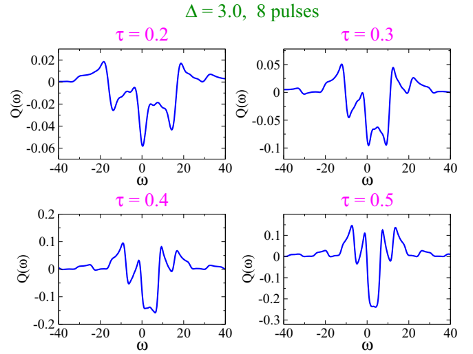
FIG. 4. Absorption spectrum of a two-level system with detuning \Delta = 3.0 driven by a periodic sequence of \pi pulses with the periods \tau = 0.2 , \tau = 0.3 , \tau = 0.4 , and \tau = 0.5 after N_p = 8 pulses. The curves present analytical results.
