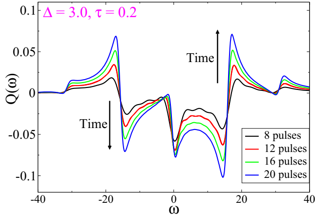
FIG. 3. Absorption spectrum of a two-level system with detuning \Delta = 3.0 , driven by a periodic sequence of \pi pulses with period \tau = 0.2 , after N_p = 8 (black), N_p = 12 (red), N_p = 16 (green), and N_p = 20 (blue) pulses. The curves present analytical results; the arrows indicate the increasing number of pulses (increasing total time of the sequence). The overall spectral shape is established early, within one to two spontaneous emission times, and at later times the peaks/dips increase in amplitude.
