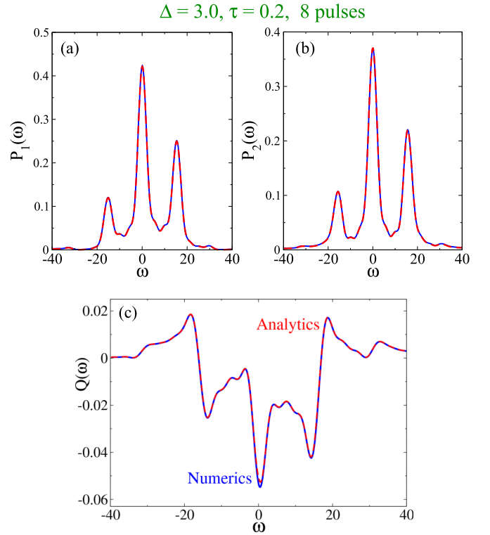
FIG. 2. Absorption spectrum of a two-level system with detuning \Delta = 3.0 driven by a periodic sequence of \pi pulses of period \tau = 0.2 after N_p = 8 pulses. Panels (a) and (b) show the terms P_1(\omega) (direct emission) and P_2(\omega) (direct absorption), correspondingly, and panel (c) shows the difference between the two terms, which is the total absorption Q(\omega) . The results are obtained by solving the master equation numerically (blue solid line) and analytically in the limit of a large number of pulses (red dashed line). The two approaches give very close results despite the assumed limit N_p \gg 1 in the analytical result and finite time step used in the Fourier transform of the numerical results.
