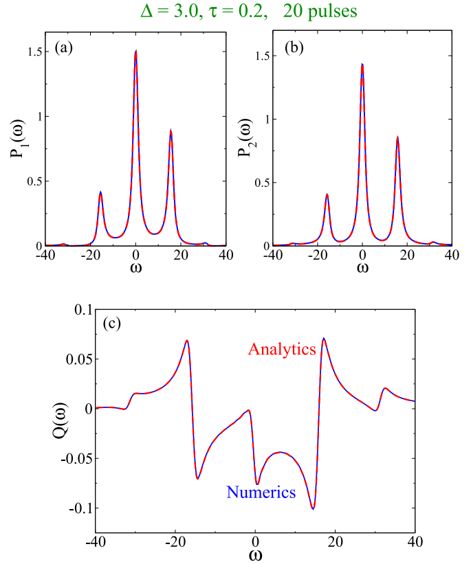
FIG. 7. Absorption spectrum of a two-level system with detuning \Delta = 3.0 driven by a periodic sequence of \pi pulses of period \tau = 0.2 after 20 pulses. The results are obtained by solving the master equation numerically (blue solid line) or analytically in the limit of a large number of pulses (red dashed line). We see that indeed the agreement between the numerical and analytical results is better at longer times (for a large number of pulses).
