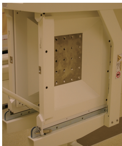
Figure 14 The UCSF 20-pinhole SPECT collimator (courtesy of Dr. Youngho Seo).
