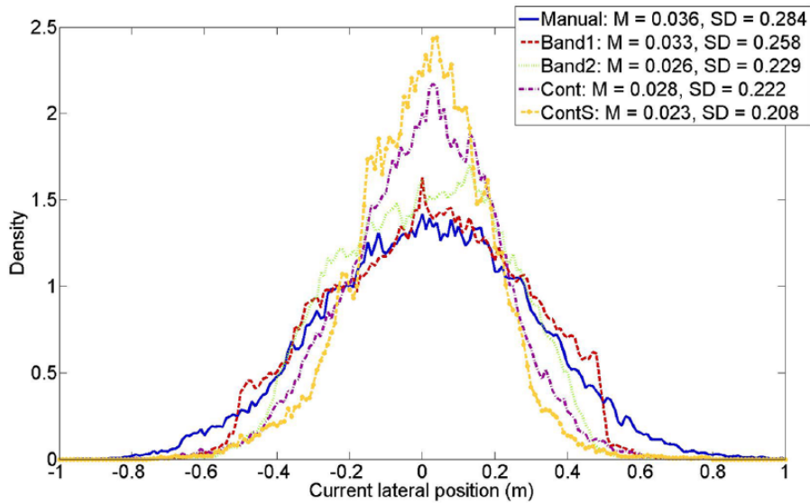
Figure 3. Distribution of the lateral position (m) over the trajectory before the shutdown moment of all participants per condition (i.e., Manual, Band1, Band2, Cont, ContS). Bins are 0.01 m. The area under each of the five curves equals 1.
