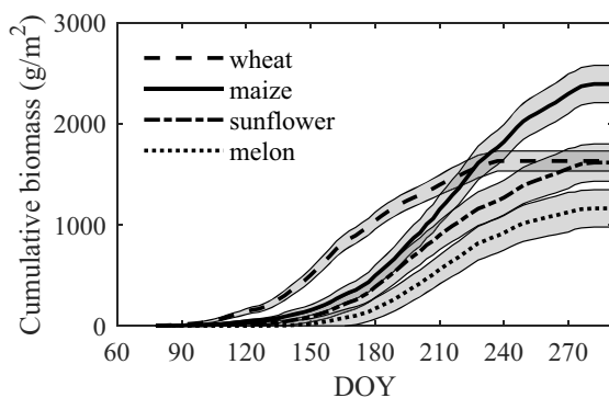
Fig. 11. Spatially averaged accumulated biomass for wheat, maize, sunflower, and melon during the growing season in the SRB in 2019; the shaded areas indicate the spatial variability with a range equal to \pm one standard deviation.
