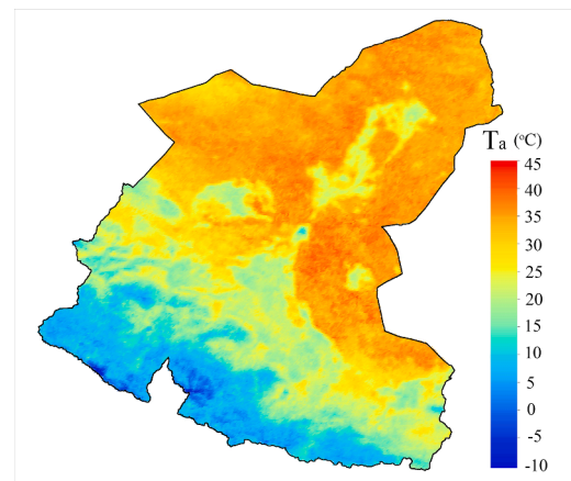
Fig. 7. Spatial variability of daily mean T_a in Jul. 14 2019 in the SRB.
