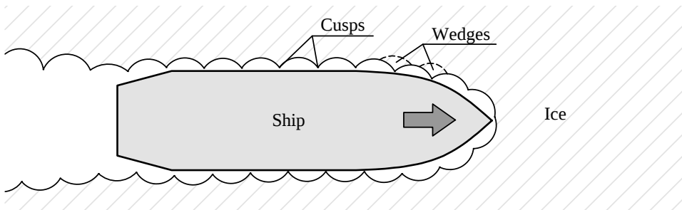
Figure 2.1: As the vessel advances, it mainly interacts with the ice sheet through a series of cusps. Each cusp fails in bending, generating wedges. This process results in an ice edge pattern that is typical for the edge tracking models.
