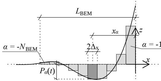
Figure 4.4: The distributed nonlinear loads, depicted with the solid curve, are approximated using a piecewise constant function. Note that \forall x > 0 the dynamic pressure is not accounted for.
