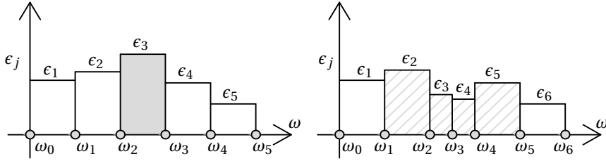
Figure B.3: An illustration of the element placement and how it affects the error contributed by element being split. The element with the largest contribution, \epsilon_3 , is split by placing a new integration point half-way the element. This results in the new situation shown on the right. The error estimates \epsilon_j of the four hatched elements are affected by the split and have to be (re)computed.
