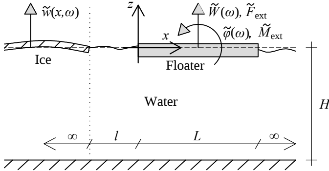
Figure 3.1: The waves generated by the floater's motion reflect at the ice-open water interface indicated by the dashed line. The reflected waves exert a pressure on the floater, altering its response.
