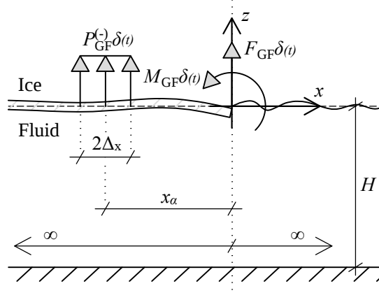
Figure 4.3: The problem definition for \tilde{\phi}_\alpha(x, z, \omega) on which the three Green's functions of the system are based.
