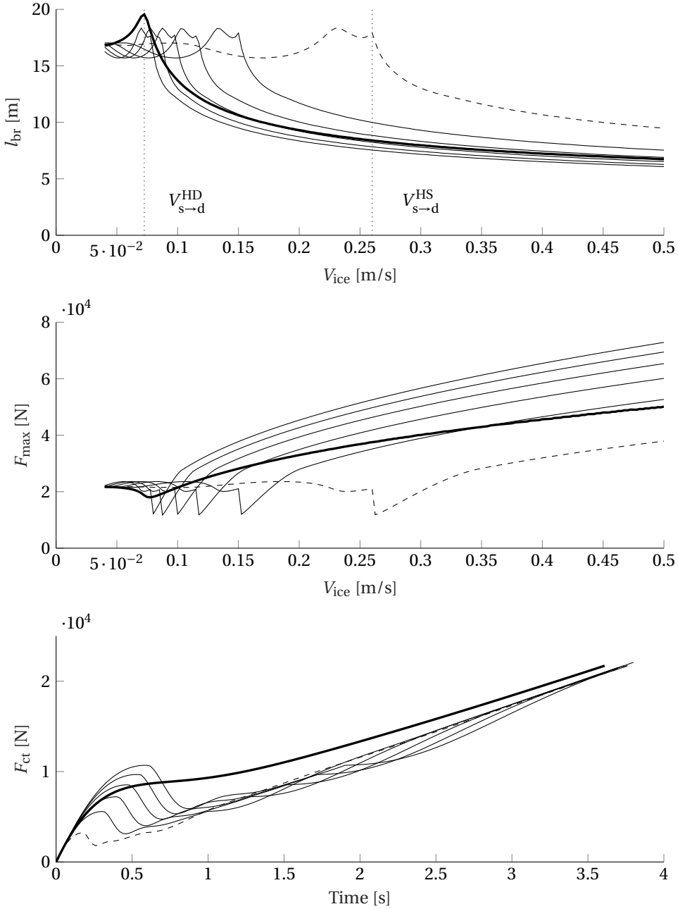
Figure 5.1: The effect of C_m on the predictions of \mathcal{M}_{eHD} . The bold curve is \mathcal{M}_{HD} . The dashed curve shows \mathcal{M}_{eHD}(\xi_d = C_{bc} = C_m = 0) = \mathcal{M}_{HS} . All subsequent solid curves are evaluations at C_m = \{2, 4, 6, 8, 10\} respectively. For the bottom graph V_{ice} = 0.04 m/s.
