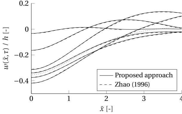
Figure 4.7: The normalized, transient, vertical response of the ice floe. The solid lines show the response of the proposed model and the dashed lines are the results from Zhao and Dempsey [202]. The lines, from top to bottom at \bar{x} = 0 , are evaluations at \tau = t\sqrt{g/l} = \{0.25, 1, 2, 8, 6, 4\} respectively. The dotted line shows the static response.
