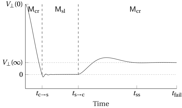
Figure 4.15: The speed at which the ice penetrates into the structure V_{pen}(t) during a typical interaction. The steady-state penetration speed V_{pen}(\infty) and a zero line are included for reference. The dashed vertical lines delimit the two modes of the contact model.
