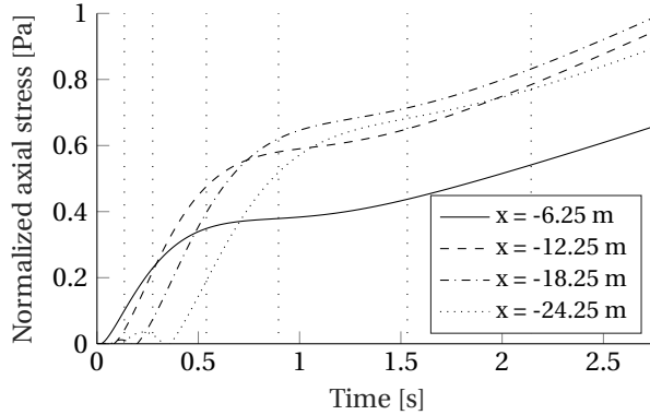
Figure 4.19: The axial stress of \mathcal{M}_{\text{HD}} normalized by the flexural yield stress \sigma_{\text{fl}} as a function of time at four locations. For this figure V_{\text{ice}} = 0.05 m/s. The vertical dotted lines indicate the failure time t_{\text{fail}} at the following ice velocities (from left to right): 0.5, 0.2, 0.1, 0.08, 0.07, 0.06 and 0.05 m/s.
