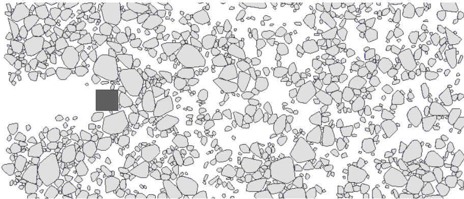
Figure 2.2: A simulation of pack ice flowing around a fixed, rectangular structure, modeled in 2D using rigid bodies without any failure modes. Image Courtesy: Marnix van den Berg.
