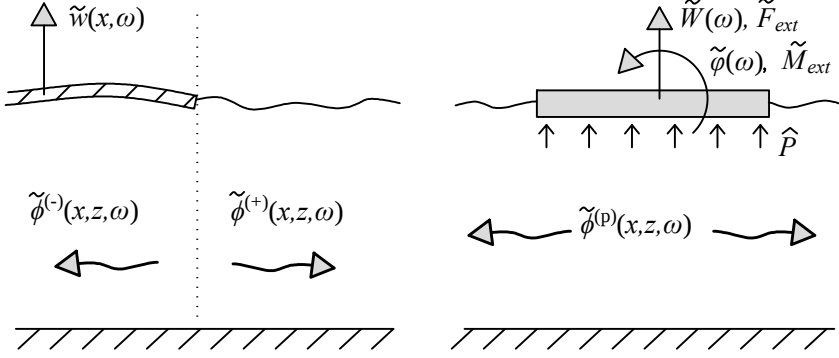
Figure 3.2: Excitation of the floater generates waves (right image) which are partly reflected and transmitted by the ice floe (left image)
