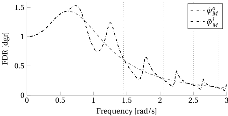
Figure 3.11: \tilde{\varphi}_M for the default parameters.
