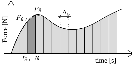
Figure 4.5: All loads are approximated as piecewise linear functions of time. The loading applied within time step \hat{n} , \hat{F}_{\hat{n}} , is highlighted.
