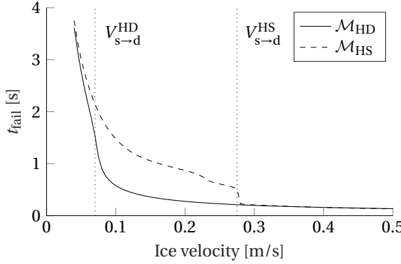
Figure 4.13: The failure time t_{\text{fail}} of both models. The vertical dotted lines indicate the transition velocity V_{s \rightarrow d} .
