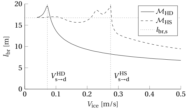
Figure 4.17: l_{br}(V_{ice}) as predicted by both models. l_{br,s} = l_{br}(0) was computed using Eq. (4.19). The dotted vertical lines indicate V_{s \rightarrow d} of each model.
