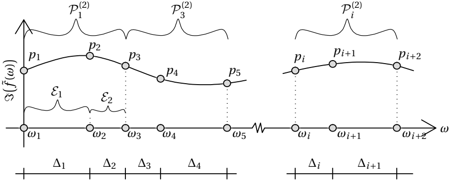
Figure B.1: \mathfrak{Z}(\tilde{f}(\omega)) is approximated using N_p second order polynomials \mathcal{P}_i^{(2)} that are indexed with i . Each polynomial is constructed using the elements \mathcal{E}_i and \mathcal{E}_{i+1} that depend on the set of points \{p_i, p_{i+1}, p_{i+2}\} .
