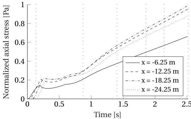
Figure 4.18: The axial stress due to bending of \mathcal{M}_{\text{HS}} normalized by the flexural yield stress \sigma_{\text{fl}} as a function of time at four locations. For this figure V_{\text{ice}} = 0.06 m/s. The vertical loosely dotted lines indicate the failure time t_{\text{fail}} at the following ice velocities (from left to right): 0.5, 0.2, 0.1, 0.08, 0.07 and 0.06 m/s.
