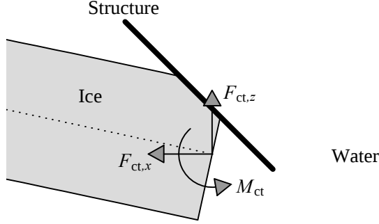
Figure 4.2: The decomposition of the contact force F_{ct} .
