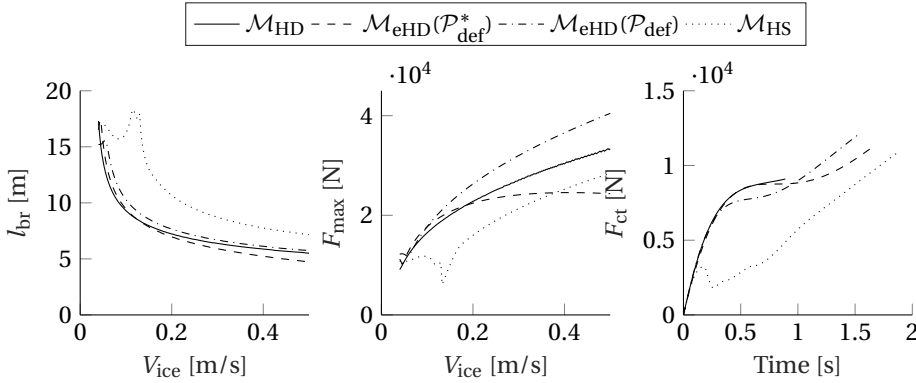
Figure 5.5: The performance of \mathcal{M}_{\text{eHD}}(\mathcal{P}_{\text{def}}) and \mathcal{M}_{\text{eHD}}^*(\mathcal{P}_{\text{def}})^* when \sigma_{\text{fl}} is changed to 250 kPa. For the right graph V_{\text{ice}} = 0.04 m/s.
