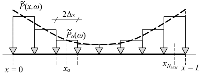
Figure 3.3: The interfacial pressure \tilde{P} is discretized using N_{\text{BEM}} = 8 elements. Within each element \alpha the pressure is constant and proportional to \tilde{P}_\alpha .
