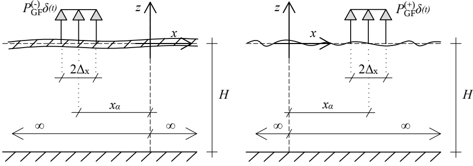
Figure A.2: The problem definition of the two complementary homogeneous infinite problems. Solving the left problem results in the ice-covered Green's function \tilde{\phi}_\alpha^{(o,p)} and the right one results in the open water Green's function \tilde{\phi}_\alpha^{(o,p)} .
