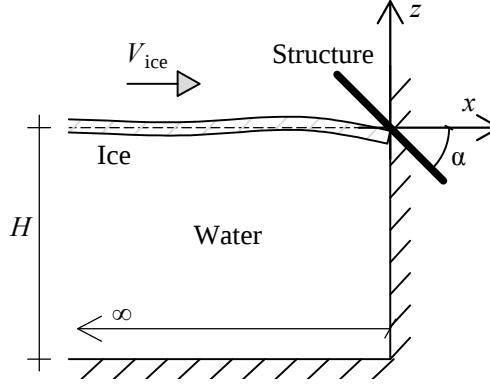
Figure 4.8: For validation a semi-infinite model is considered.
