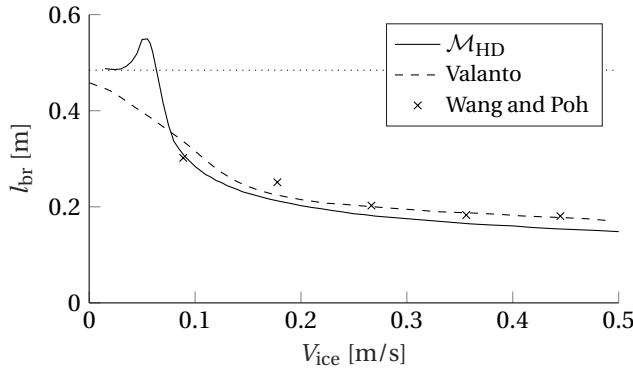
Figure 4.22: l_{br}(V_{ice}) as predicted by all three models. The horizontal dotted line is the static breaking length computed with Eq. (4.19).
