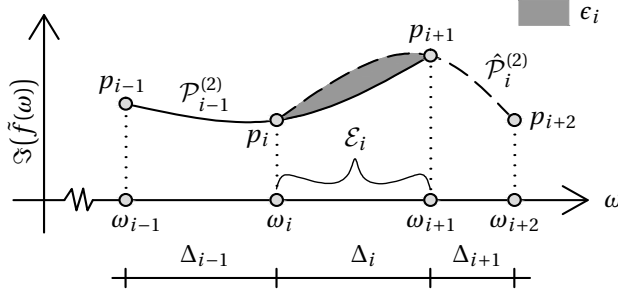
Figure B.2: The error within element i , \epsilon_i , is estimated as the gray area between \mathcal{P}_{i-1}^{(2)}(\omega) , depicted by the solid line, and \hat{\mathcal{P}}_i^{(2)}(\omega) , depicted by the dashed line.
