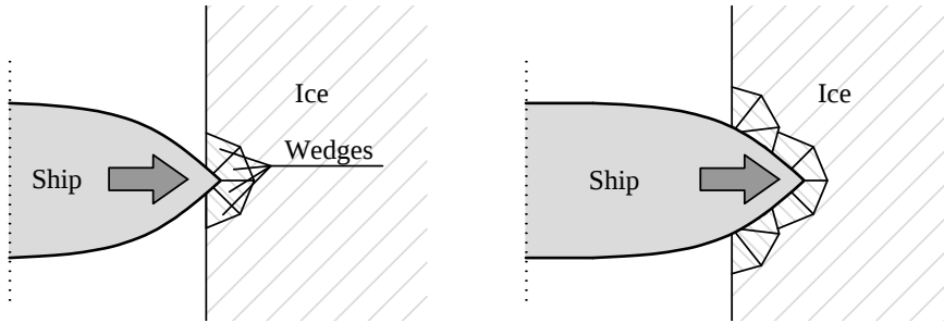
Figure 2.3: An illustration of an analytical failure model that assumes that each interaction point ultimately leads to bending failure, initiating both radial and circumferential cracks, thereby generating an assumed number of wedges. As the vessel advances, the previously generated wedges are pushed below the ship and the failure process repeats itself.
