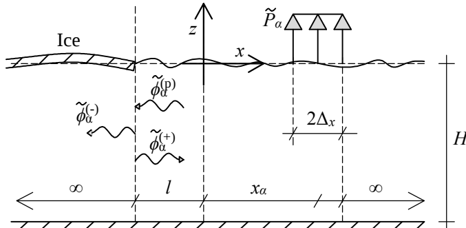
Figure 3.4: The generation of a transmitted potential \tilde{\phi}_\alpha^{(-)} and reflected potential \tilde{\phi}_\alpha^{(+)} due to the presence of the ice.
