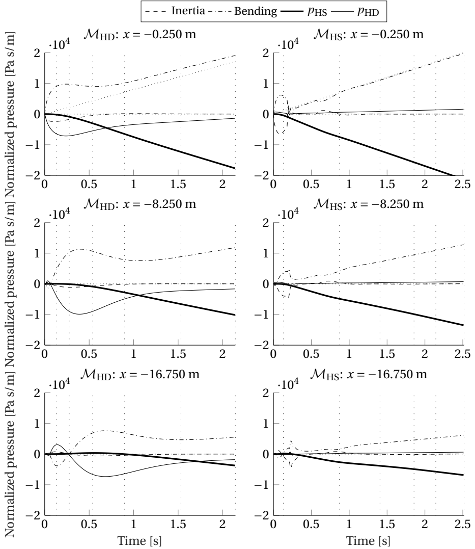
Figure 4.12: The four important factors that act on the ice floe at three locations, normalized by the ice velocity. A zero-line and the static bending pressure are included for reference with the dotted sloped lines. The vertical loosely dotted lines indicate the failure time t_{fail} at the following ice velocities (from left to right): 0.5, 0.2, 0.1, 0.08, 0.07 and 0.06 m/s.
