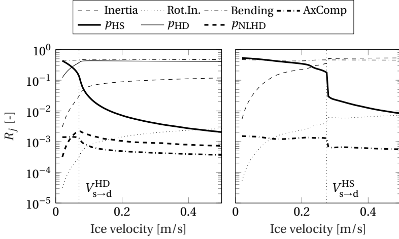
Figure 4.11: The relative importance R_j of all seven terms. Left: \mathcal{M}_{\text{HD}} . Right: \mathcal{M}_{\text{HS}} . The vertical dotted lines indicate the transition velocity V_{s \rightarrow d} that separates the quasi-static and dynamic interactions. V_{s \rightarrow d} is discussed in detail in Sec. 4.3.3.
