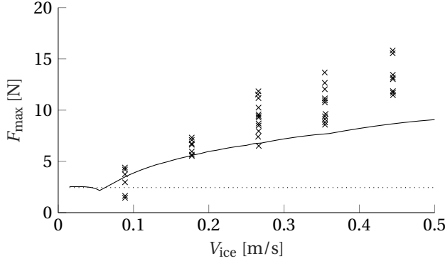
Figure 4.10: F_{\max} for a range of ice velocities. The crosses show the experimental data. The values predicted by the proposed model are shown by the curve. The dotted line is the static F_{\max} .
