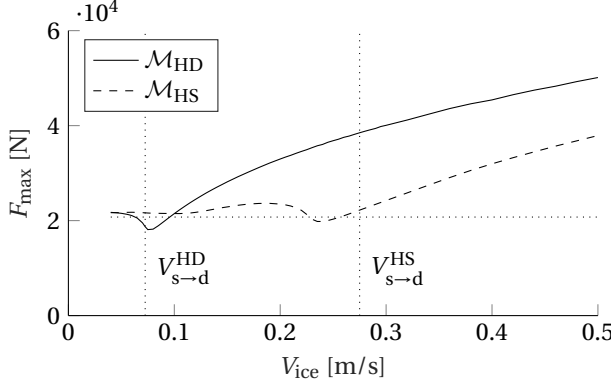
Figure 4.20: F_{max}(V_{ice}) of both models. The static force is included for reference as is depicted with the dotted horizontal line.
