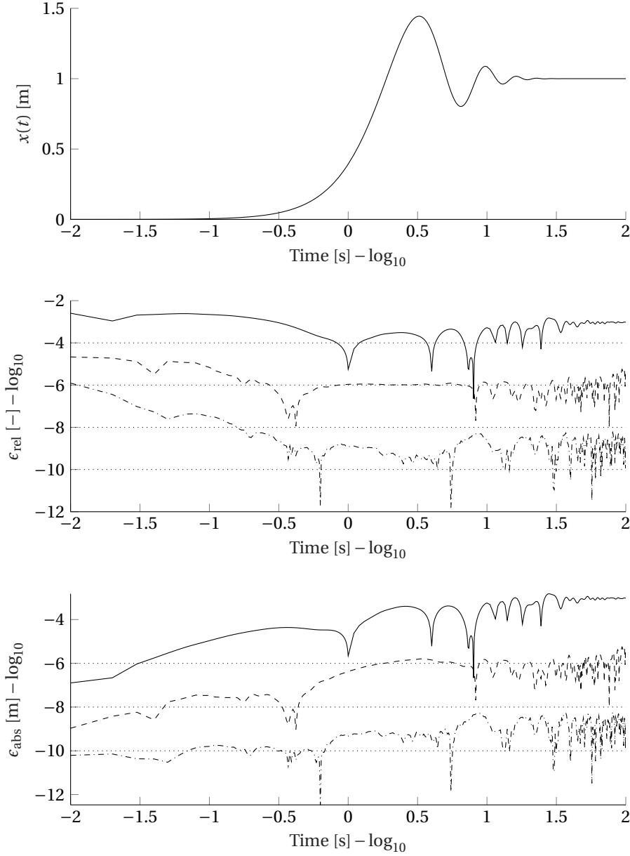
Figure B.4: The displacement x(t) for three sets of tolerances: \{\epsilon_{\text{rel}} = 10^{-2}, \epsilon_{\text{abs}} = 10^{-4}\} solid line, \{\epsilon_{\text{rel}} = 10^{-4}, \epsilon_{\text{abs}} = 10^{-6}\} dashed line, \{\epsilon_{\text{rel}} = 10^{-6}, \epsilon_{\text{abs}} = 10^{-8}\} dash-dot line.
