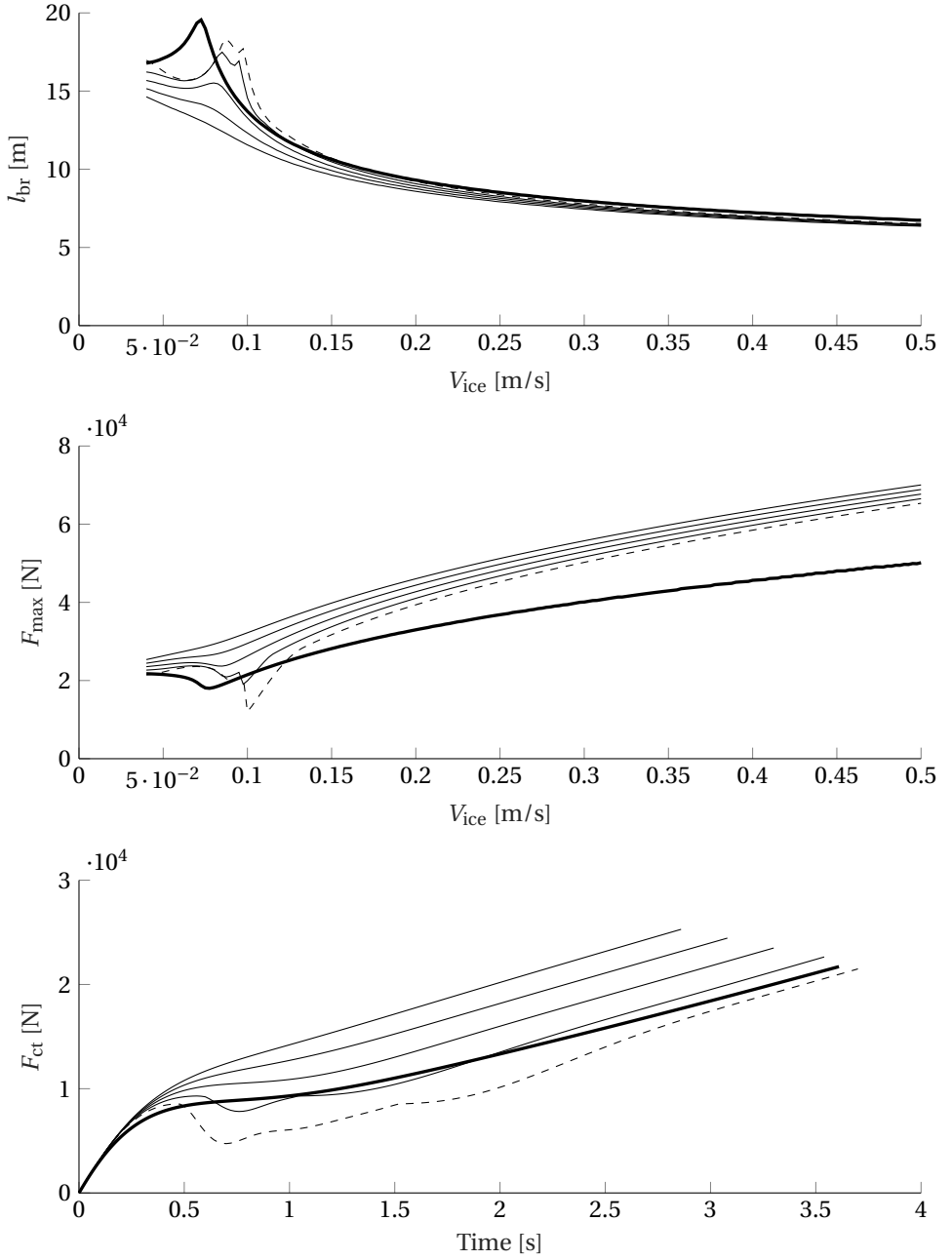
Figure 5.2: The effect of \xi_d on the predictions of \mathcal{M}_{eHD} . The bold curve is \mathcal{M}_{HD} . The dashed curve shows \mathcal{M}_{eHD}(\{C_m = 6.26, \xi_d = C_{bc} = 0\}) \neq \mathcal{M}_{HS} . All subsequent solid curves are evaluations at \xi_d = \{1, 2, 3, 4\} respectively. For the bottom graph V_{ice} = 0.04 m/s.
