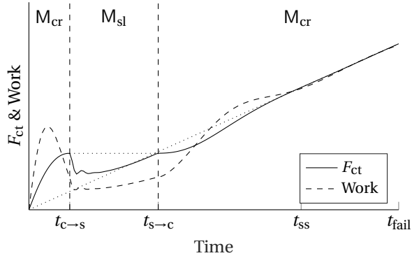
Figure 4.14: An illustration of how the contact force F_{ct} , depicted with the solid curve, develops during a typical interaction. The work done by the contact force is shown by the dashed curve. Both signals are normalized. The contact force based on a static equilibrium is depicted with the dotted diagonal line. The dashed vertical lines delimit the two modes of the contact model.
