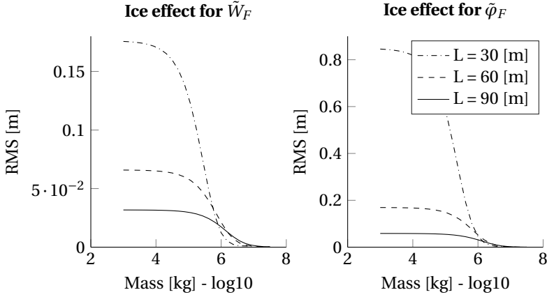
Figure 3.8: The effect of the floater's mass on the ice effect.
