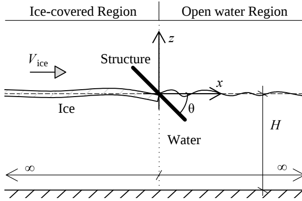
Figure 4.1: A sketch of the 2D semi-analytical ISI model \mathcal{M}_{HD} that includes hydrodynamics. The region x \leq 0 is referred to as the ice-covered region and the region x > 0 as the open water region.
