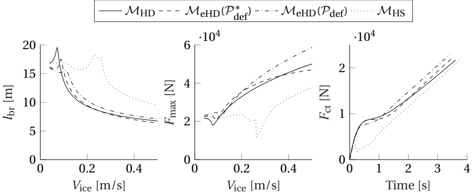
Figure 5.4: The performance of \mathcal{M}_{\text{eHD}}(\mathcal{P}_{\text{def}}) and \mathcal{M}_{\text{eHD}}(\mathcal{P}_{\text{def}}^*) . For the right graph V_{\text{ice}} = 0.04 \text{ m/s} .
