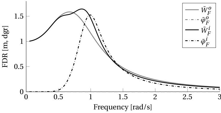
Figure 3.10: The main peak of the FDR is amplified when l = 0 .
