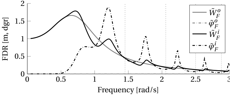
Figure 3.5: The vertical lines are related to the recurrence rate of the peaks and is discussed later. \tilde{\varphi}_F^o is zero as the problem is symmetric when no ice is present.
