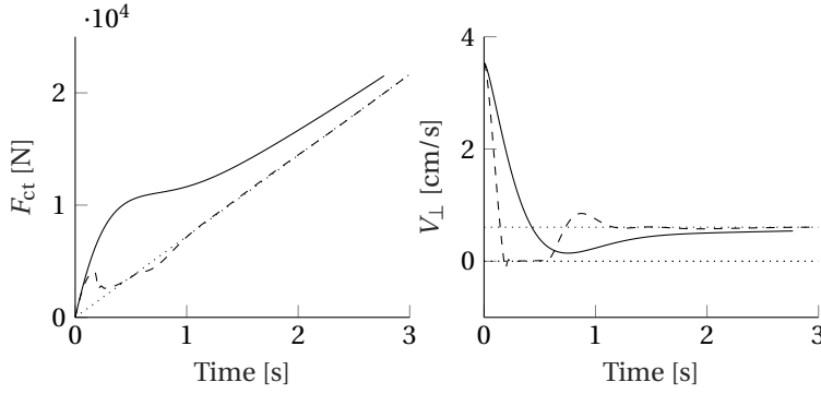
Figure 4.16: F_{ct}(t) (left) and V_{\perp}(t) (right) for \mathcal{M}_{HS} (dashed) and \mathcal{M}_{HD} (solid). The dotted line on the left shows the static contact force. On the right a zero line and V_{\perp}(\infty) are included for reference. V_{ice} was set to 0.05 m/s for this figure.
