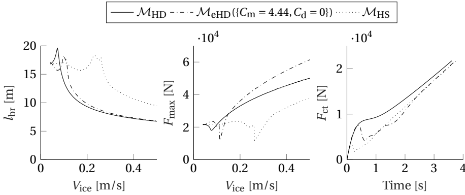
Figure 5.6: The performance of \mathcal{M}_{eHD}(\{C_m = 4.44, \xi_d = C_{bc} = 0\}) for the default set of parameters. For the right graph V_{ice} = 0.04 m/s.
