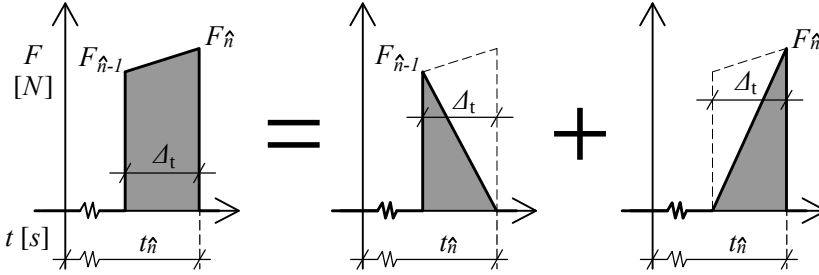
Figure 4.6: The loading applied within a single time-step \hat{F}_{\hat{n}}(t, q_{\hat{n}}) is decomposed into two parts: one proportional to F_{\hat{n}-1} and the other proportional to F_{\hat{n}} .
