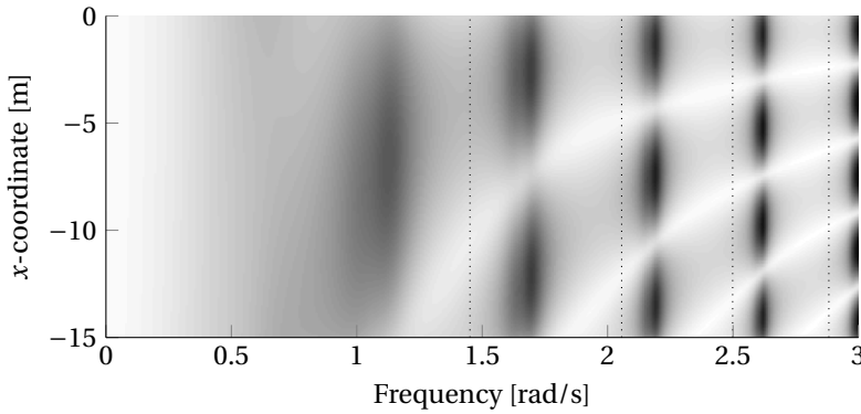
Figure 3.7: The surface amplitude within the gap for different frequencies. White represents a small amplitude, while black represents a large one.
