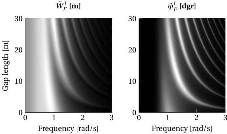
Figure 3.9: The effect of the gap length l on the response with nearby ice. White is a large amplitude and black a small.
