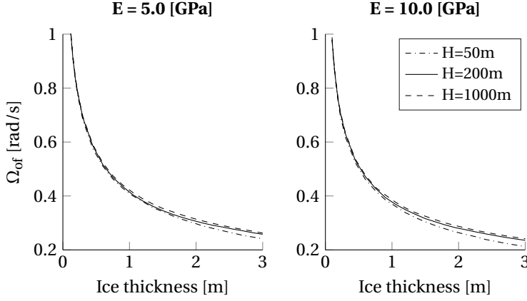
Figure 3.6: \Omega_{of} for a range of ice parameters.
