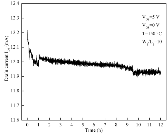
Figure 2. Continuous drain current ( I_{DS} ) measurement during 12 h burn-in period. constant value, ready for gas testing.
