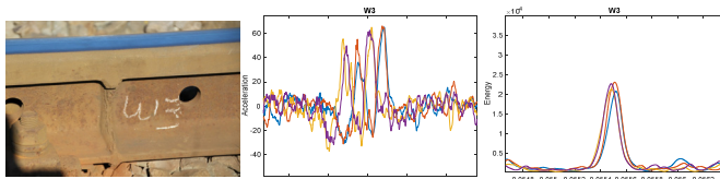
Figure 2. Example of measurements on a weld, a) photo of the weld, b) ABA in the time domain at the weld, c) energy due to weld-wheel impact.
