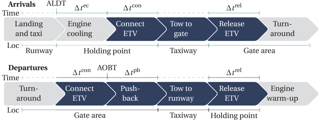
Figure 4.2.: Towing process for departing/arriving aircraft. An ETV is connected to an aircraft in the green time blocks [31].
